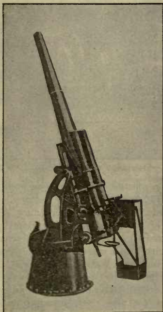
NO. 6.—EHRHARDT 65 MM. ANTI-BALLOON GUN L-35.
