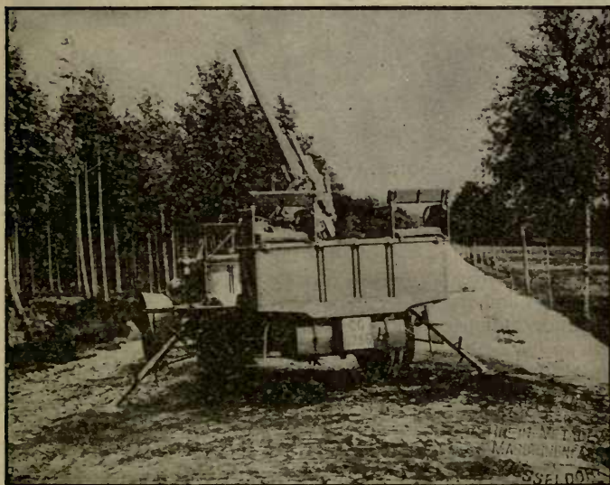
No. 9.—EHRHARDT 65 MM. ANTI-BALLOON GUN.
