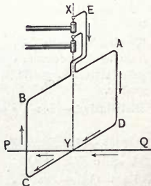
Fig. 220. Electro-Dynamic Attraction.
