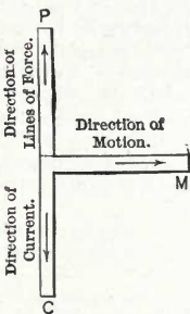
Fig. 304. Fleming's Rule.
