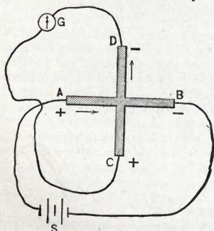
Fig. 226. Hall Effect.
