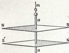
Fig. 402. Astatic Needle.
