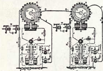
Fig. 543. Delany's Synchronous Multiplex Telegraph.
