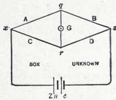
Fig. 77. Electric Balance.
