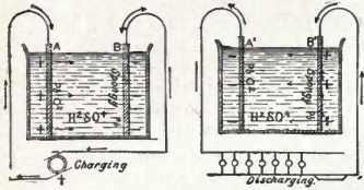
Figs. 101 and 102. Storage Cell.
