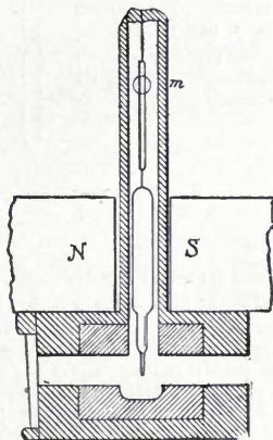
Fig. 457. Boys' Radio-Micrometer.
