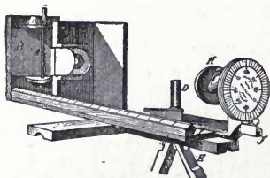
Fig. 428. Ayrton & Perry's Dispersion Photometer.
