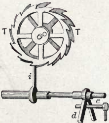
Fig. 540. Step-by-Step Wheel.
