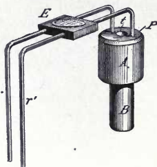
Fig. 148. Standard Ohm.
