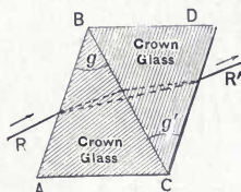
Fig. 342. Equal and Opposite Refracting Angles.
