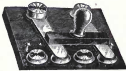
Fig. 523. Pole-Changing Switch.
