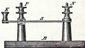
Fig. 329. Short-Circuit Key.
