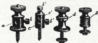
Fig. 448. Binding Posts.
