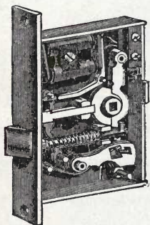
Fig. 347. Electric Lock.
