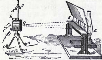
Fig. 274. Mirror Galvanometer.
