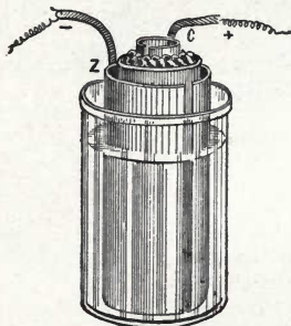
Fig 106. Daniell's Cell.
