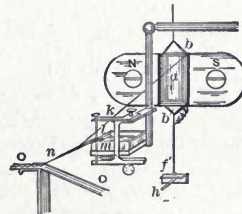
Fig. 469. The Siphon Recorder.
