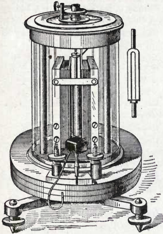
Fig. 278. Torsion Galvanometer.
