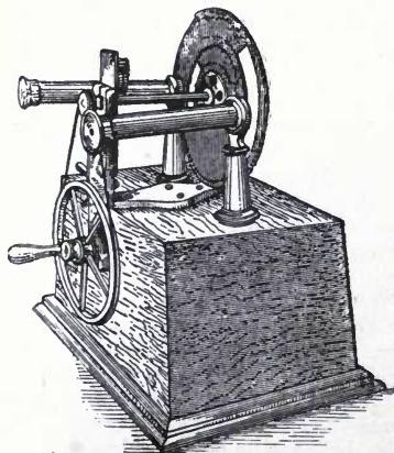
Fig. 431. Varley's Photometer.
