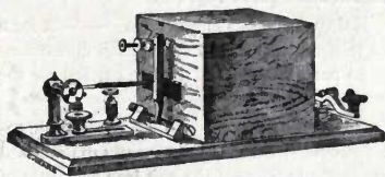
Fig. 479. Box-Sounding Relay
