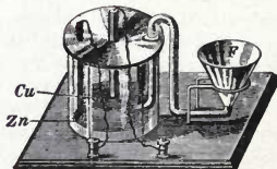
Fig. 119. Thomson's Form of Daniell's Cell.
