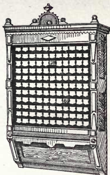
Fig. 14. Electro-Magnetic Annunciator.
