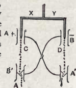
Fig. 3. Water-Drop Charging Accumulator.
