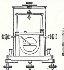
Fig. 270. Nalder's Galvanometer.
