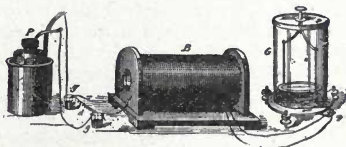
Fig. 300. Mutual Induction.
