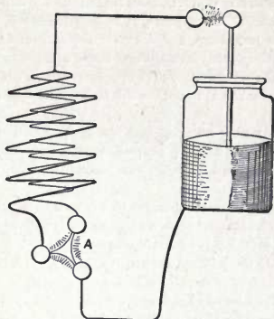
Fig. 513. Apparatus for T and Y Shaped Sparks.
