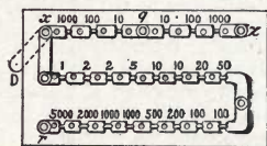
Fig. 75. Box Balance.
