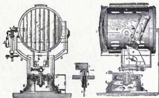
Fig. 452. Mangin Projector.
