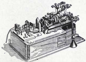
Fig. 423. Edison's Improved Phonograph.
