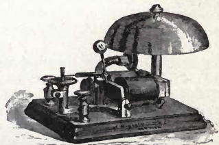
Fig. 47. Single-Stroke Bell.
