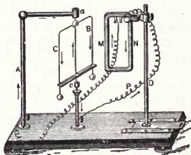
Fig. 219. Ampère's Stand.
