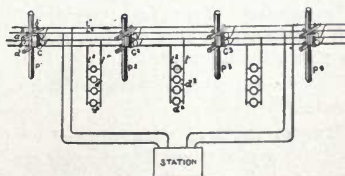
Fig. 557. Transformer Circuits.
