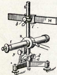
Fig. 552. Reading Telescope.
