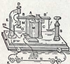
Fig. 478. Telegraphic Relay, German Pattern.
