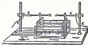
Fig. 490. Apparatus for Measuring Resistance of Liquid.
