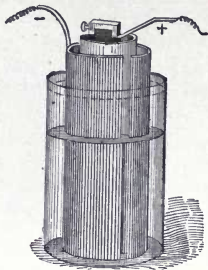
Fig. 105. Bunsen Cell.
