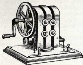
Fig. 362. Magneto-Electric Machine.
