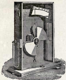
Fig. 564. Vertical electrostatic voltmeter.
