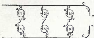
Fig. 130. Multiple-Series-Connected Cells.
