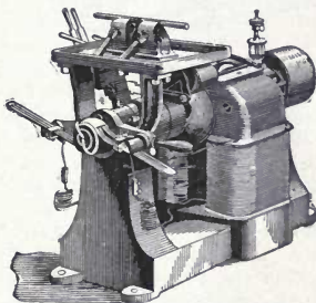
Fig. 566. The Thomson Direct Welder.
