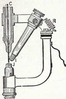
Fig. 337. Semi-Incandescent Lamp.
