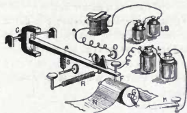
Fig. 399. Electro-Motograph .
