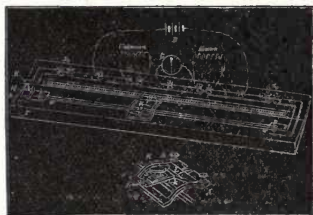
Fig. 79. Slide Form of Bridge.
