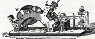
Fig. 468. Morse Recorder.
