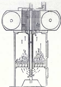
Fig. 400. Pyromagnetic Motor.
