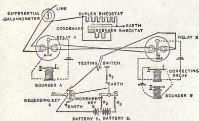
Fig. 534. Quadruplex Telegraphy, Differential Method.
