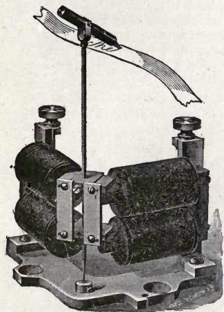
Fig. 548. Receiver of Writing Telegraph.
