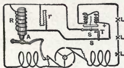
Fig. 474. Thomson-Houston Regulator.
