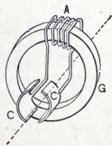
Fig. 158. Two-part Commutator.
