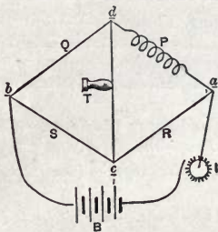
Fig. 80. Inductance Bridge.
