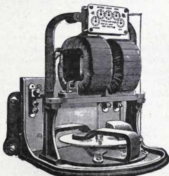
Fig. 396. Watt Meter.
