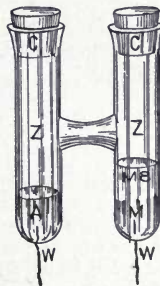
Fig. 115. Clark's Standard Cell.
