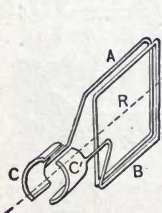
Fig. 157. Two-part Commutator.
