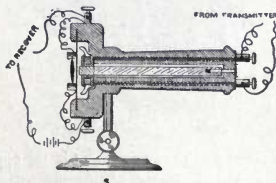
Fig. 481. Microphone Relay.
