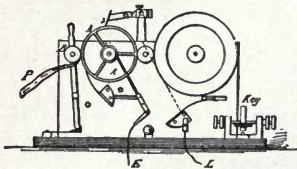
Fig. 467. Bain Recorder.
