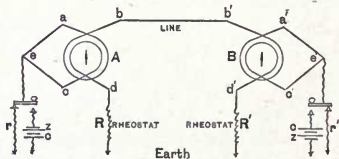
Fig. 529. Duplex Telegraphy, Differential Method.
