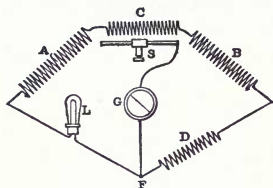
Fig. 297. Edison-Howell Lamp Indicator.
