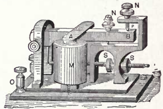
Fig 510. Morse Sounder.
