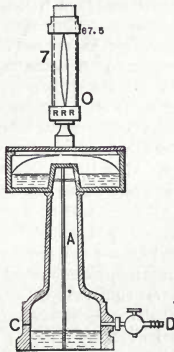
Fig. 317. Carcel Candle Burner.
