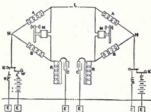
Fig. 528. Duplex Telegraphy, Bridge, Method.
