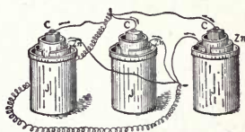
Fig. 128. Batteries connected in a Multiple Circuit.
