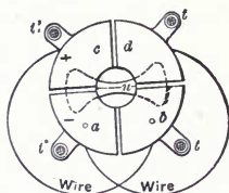
Fig. 232. Quadrant Electrometer.
