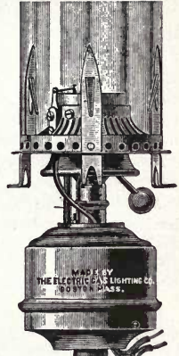
Fig. 85. Argand Electric Burner.
