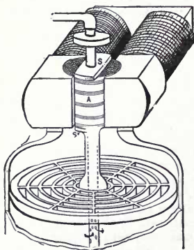
Fig. 401. Pyromagnetic Motor.
