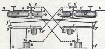
Fig. 485. Hick's Automatic Button Repeater.
