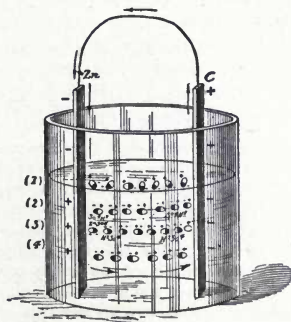
Fig. 293. Grothüss' Hypothesis of Electrolytic Polarization.
