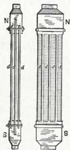
Fig. 367. Compound Magnet.
