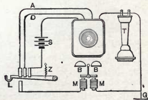
Fig. 525. Automatic Telephone Switch.
