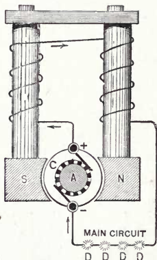
Fig. 354. Series Dynamo.
