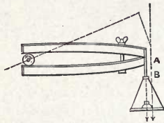
Fig. 70. Prony Brake.
