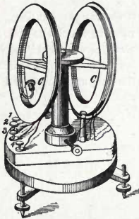
Fig. 273. Differential Galvanometer.
