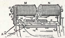
Fig. 496. Magneto-Optic Rotation.
