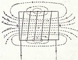
Fig. 374. Direction of Lines of Force.
