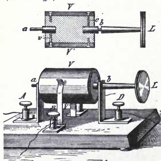
Fig. 160. Ruhmkorff's Commutator.
