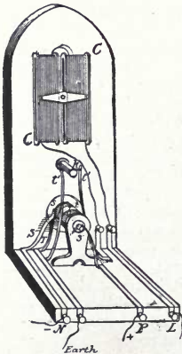
Fig. 536. Wheatstone and Cooke's Single-Needle Apparatus, Internal Arrangement.
