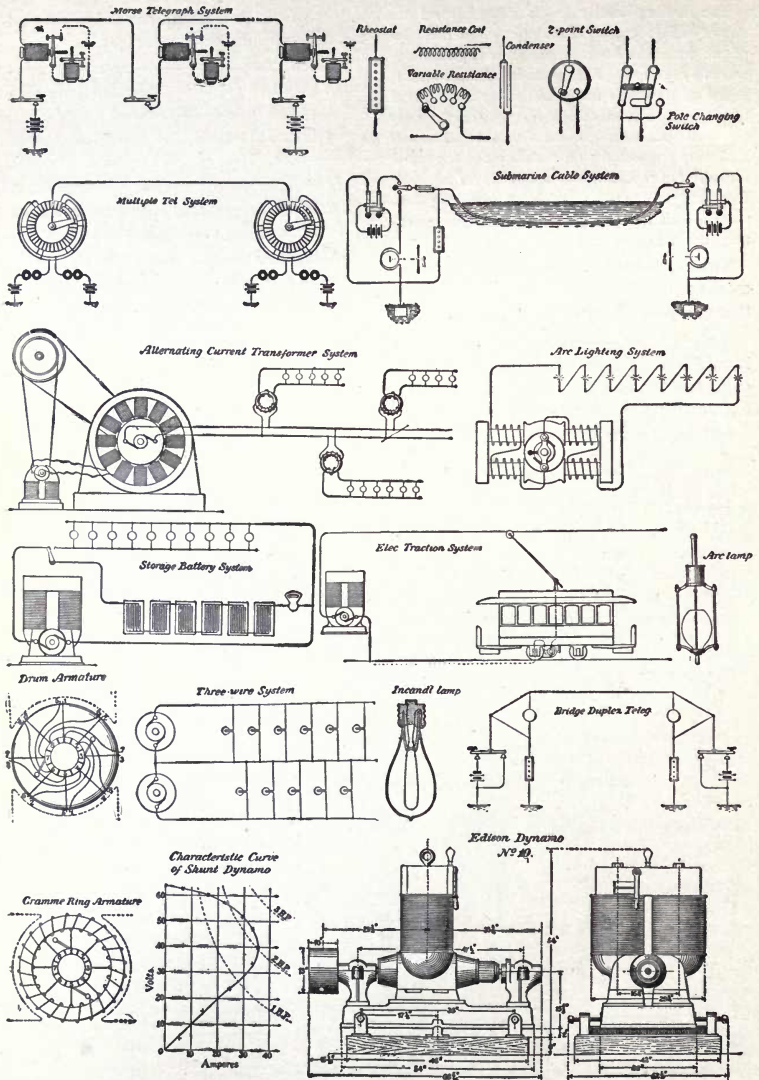
Fig. 520. Crocker's Chart of Standard Electric Symbols and Diagrams.
