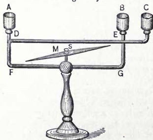
Fig. 265. Ampere's Apparatus.
