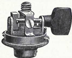
Fig. 522. Lamp-Socket Switch.
