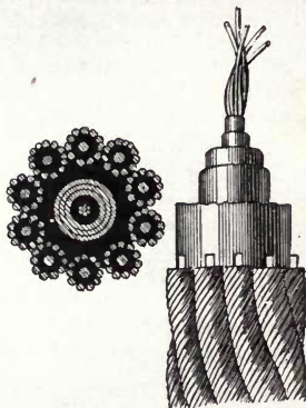
Fig. 94. Electric Cable.
