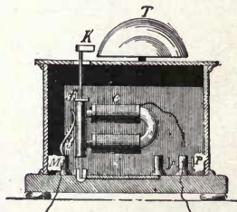
Fig. 8. Automatic Make-and-Break.
