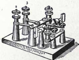
Fig. 328. Reversing Key.
