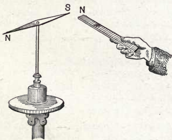
Fig. 30. Magnetic Attraction.
