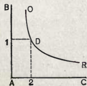
Fig. 1. Axes of Co-ordinates.
