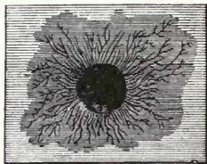
Fig. 254. Lichtenberg's Dust Figures.
