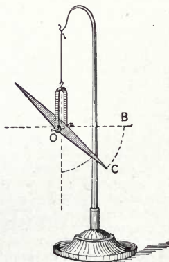
Fig. 406. Dipping Needle.
