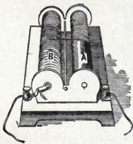
Fig. 494. Wheatstone's Rheostat.
