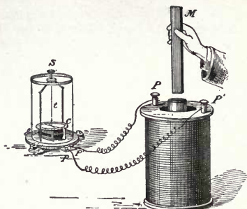
Fig. 302. Magneto-Electric Induction.
