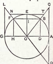
Fig. 261. Trigonometrical Functions.
