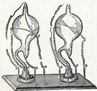
Fig. 394. Effects of Molecular Bombardment.
