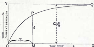
Fig. 191. Logarithmic Curve.
