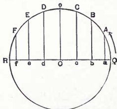
Fig. 398. Simple-Harmonic Motion.
