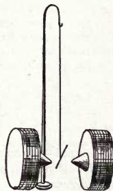
Fig. 415. Diamagnetic Polarity
