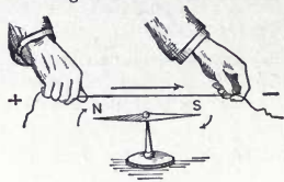
Fig. 264. Oersted's Experiment.
