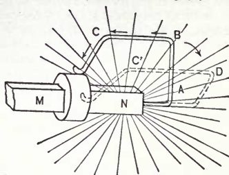
Fig. 309. Unipolar Induction.
