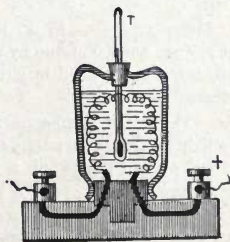
Fig. 97. Electric Calorimeter.
