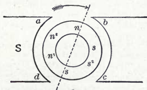
Fig. 292. Horns of Dynamo.
