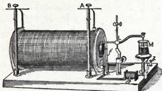
Fig. 142. Ruhmkorff Coil.
