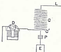
Fig. 26. Counter-Electromotive Force Lightning Arrester.
