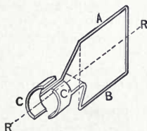
Fig. 156. Two-part Commutator.
