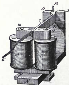
Fig. 482. Polarized Relay.
