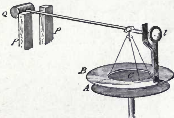
Fig. 230. Attracted-Disc Electrometer.
