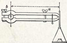
Fig. 71. Prony Brake.
