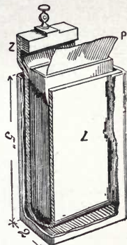
Fig. 110. Grove's Cell.
