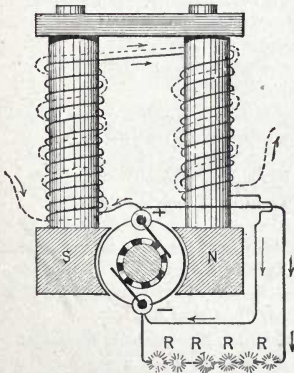
Fig. 356. Shunt and Separately Excited Dynamo.
