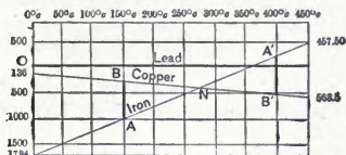
Fig. 198. Thermo-Electric Diagram.
