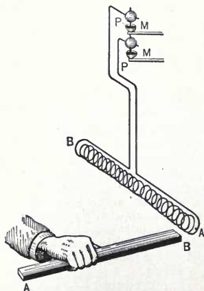
Fig. 505. Practical Solenoid.
