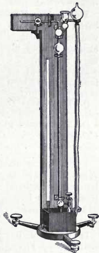
Fig. 454. Geissler's Mercurial Air Pump.
