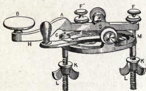
Fig. 531. Telegraphic Key.
