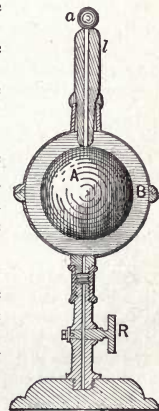
Fig 99. Condenser.
