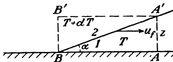
FIG. 53.—Static effect of the frontal passage on the surface pressure.
