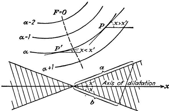
FIG. 74.—Frontogenetical and frontolytical sectors. (After Petterssen.)
