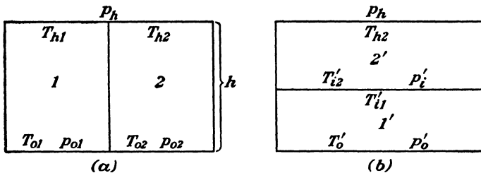
FIG. 66.—Rearrangement of two air masses of different temperature. (After Margules.)
