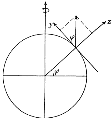
FIG. 30.—The direction cosines of the earth's axis.
