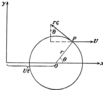
FIG. 46.—Superposition of straight and circular motion.
