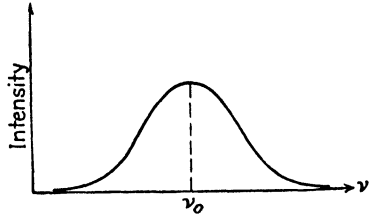
FIG. 20.—Energy distribution in a spectral line.
