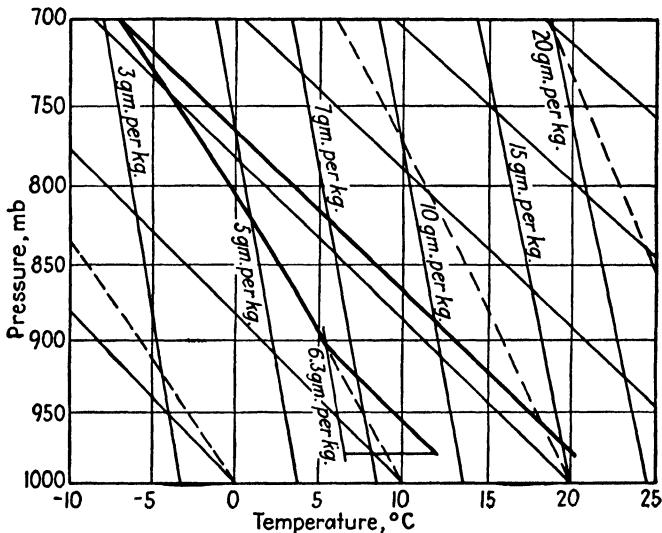
FIG. 8.—Pseudo-adiabatic chart.
