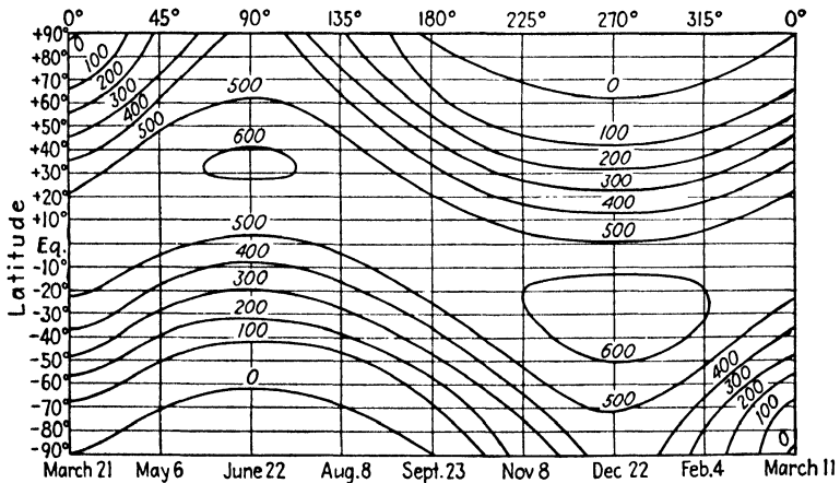
FIG. 19.—Daily insolation in calories per square centimeter received at the earth’s surface when the atmospheric transmission coefficient is 0.7. (After Milankovič’s computations.)
