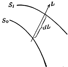
FIG. 55.—Velocity of a characteristic curve.
