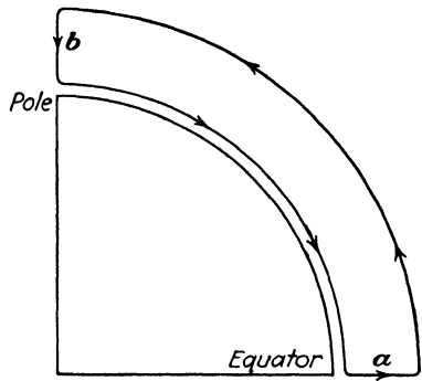
Fig. 68.—Circulation on a non-rotating earth.
