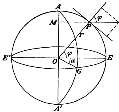
FIG. 27.—Acceleration in spherical coordinates.
