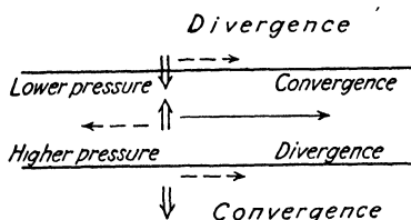
FIG. 65.—Effect of lateral mixing on a current through a fluid at rest.
