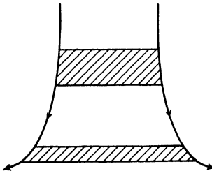
FIG. 4.—Subsiding motion and shrinking.
