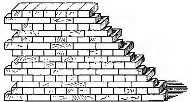
EUROPEAN BRICK-WORK.
