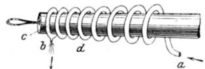
a = Dampfeinströmung, b = Dampfausströmung, c = kleinster Formring, d = mittlerer Formring.
