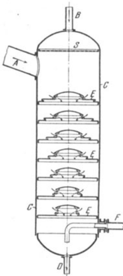
Fig. 144. Apollo-Kühler.
