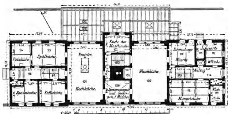
Erdgeschoss.
