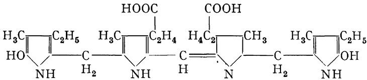
Urobilin ( C_{33}H_{42}N_6O_4 ).
