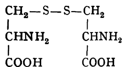
Cystin
