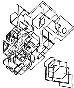
Abb. 63. Salpetersaurer Harnstoff.
