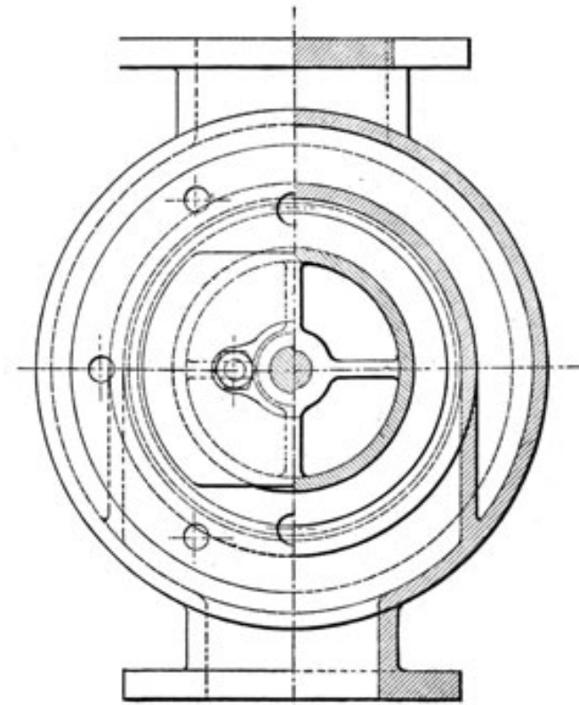
REVERSING VALVE FOR STEAM CAPSTANS
