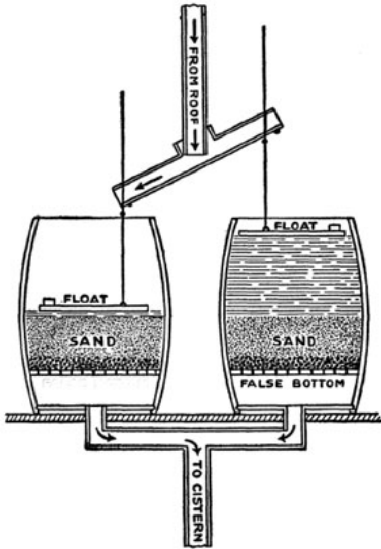
TWO-BARREL FILTER
