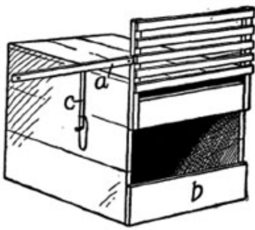
TRAP NEST
