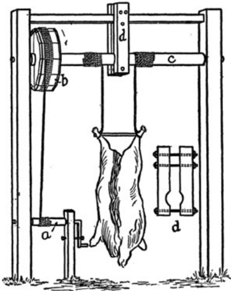
CARCASS DERRICK
