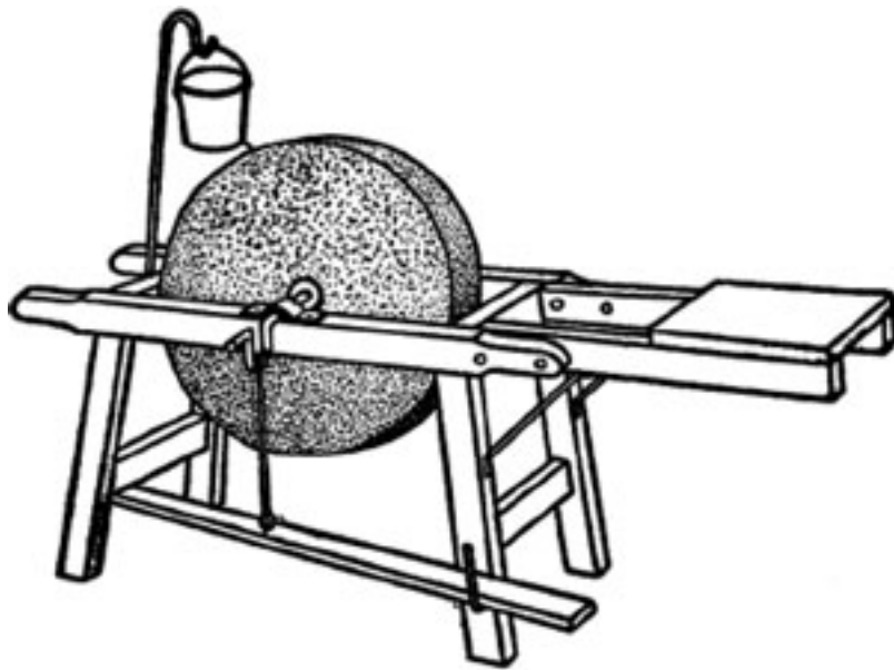
HANDY GRINDSTONE RIG
