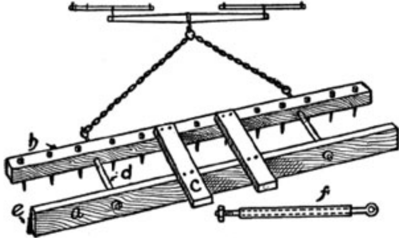
HARROWS AND LEVELS AT ONCE
