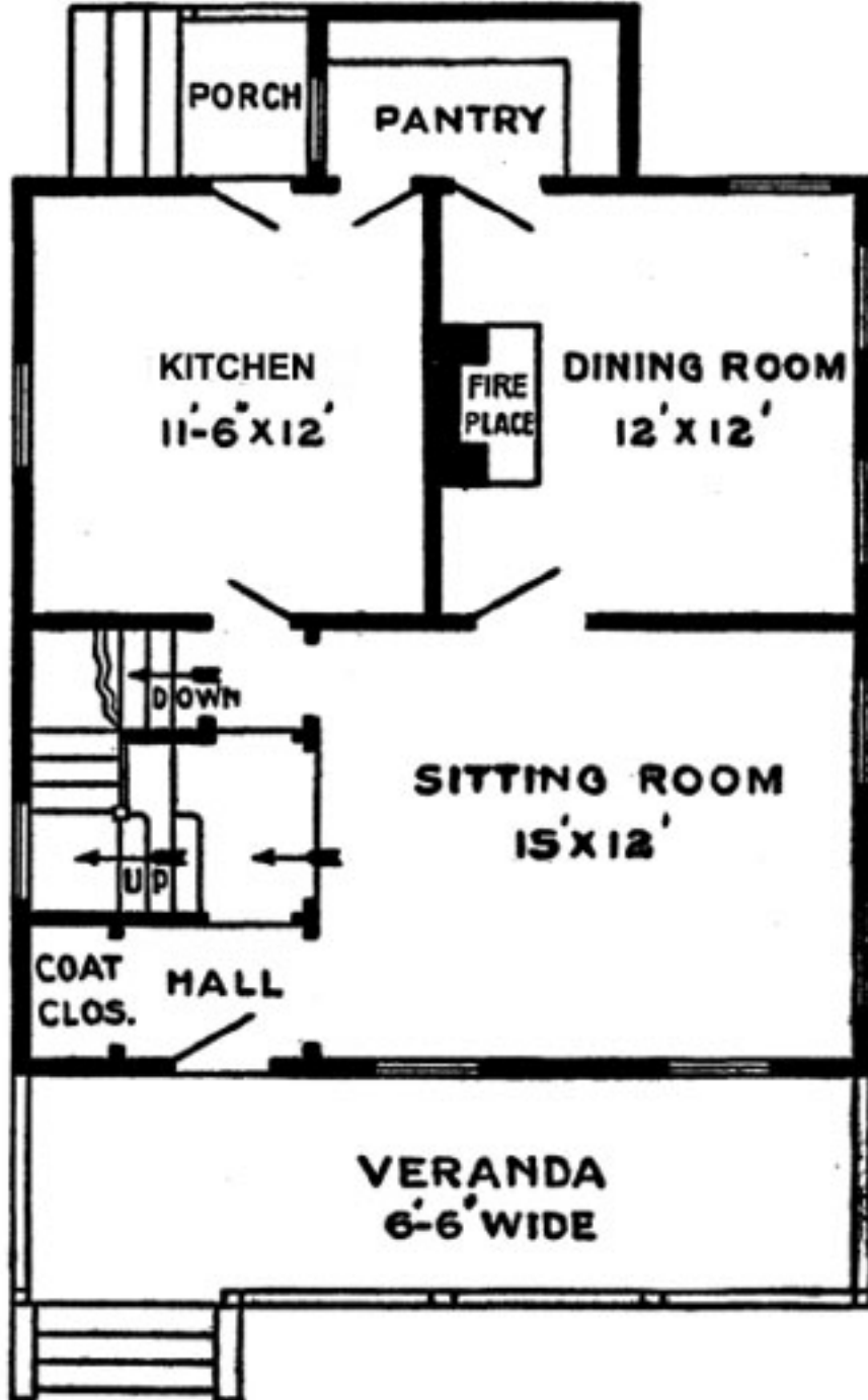
FIRST FLOOR COTTAGE PLAN
