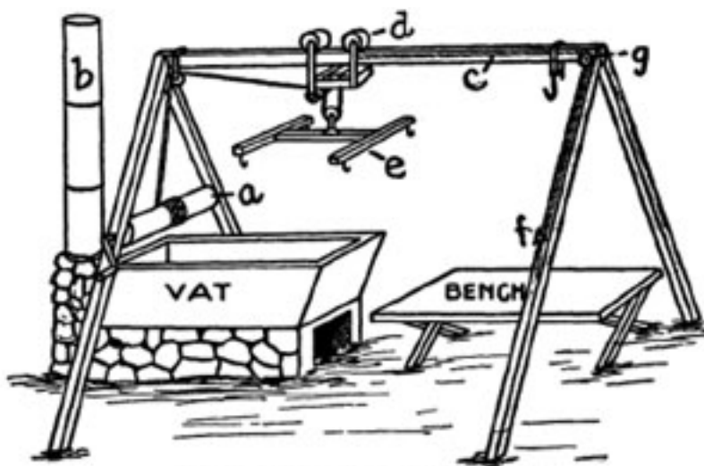
ONE-MAN BUTCHERING RIG
