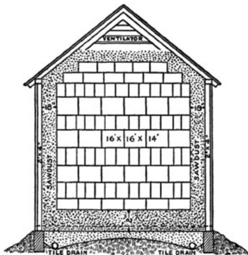
CROSS-SECTION OF ICEHOUSE
