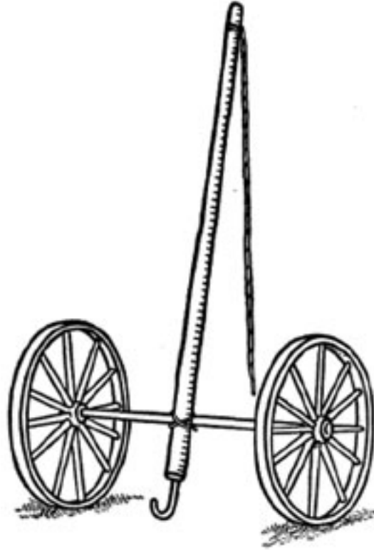
FIGURE 2—HOOK AND TRUCK
