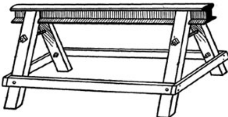
RAIL ANVIL
