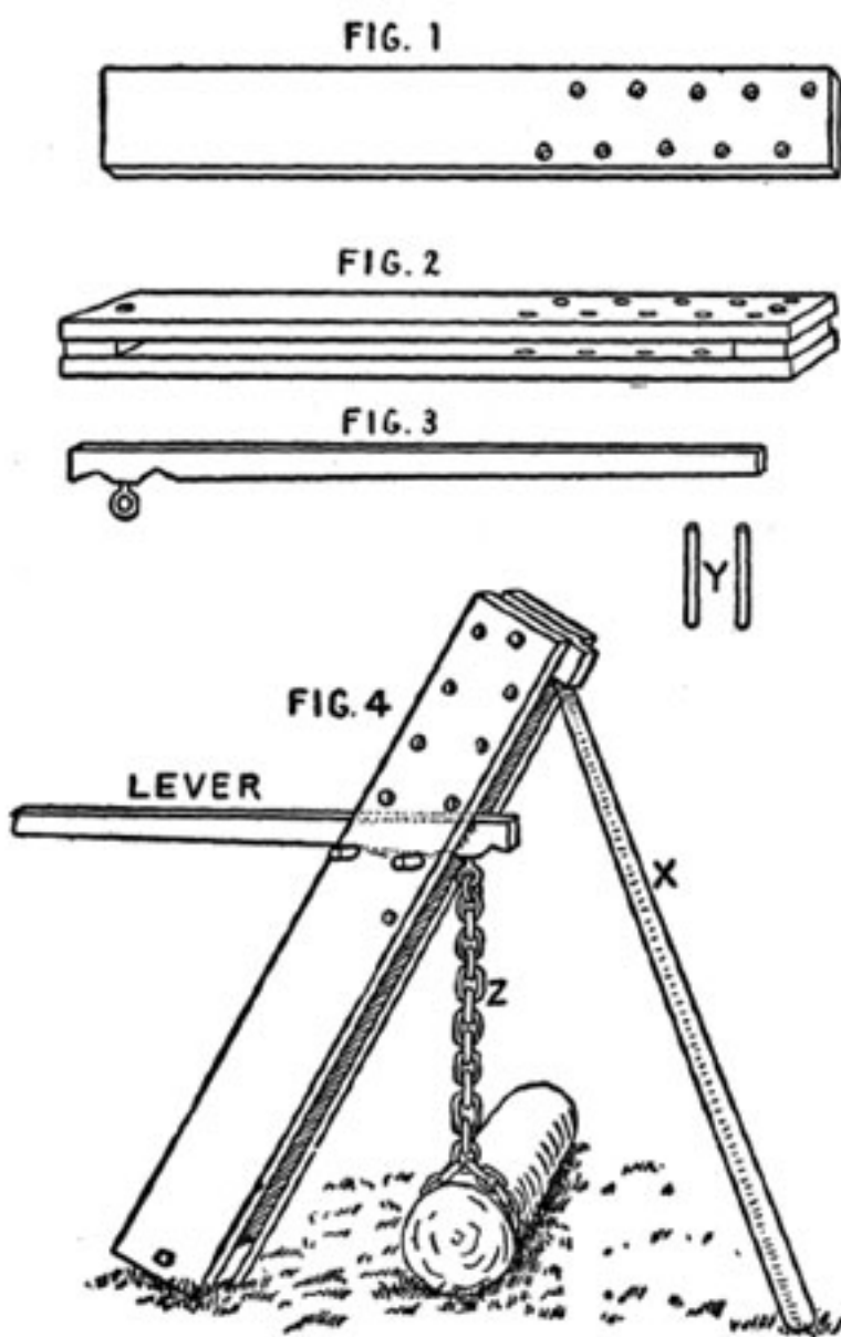
WEIGHT LIFTER AND DETAILS
