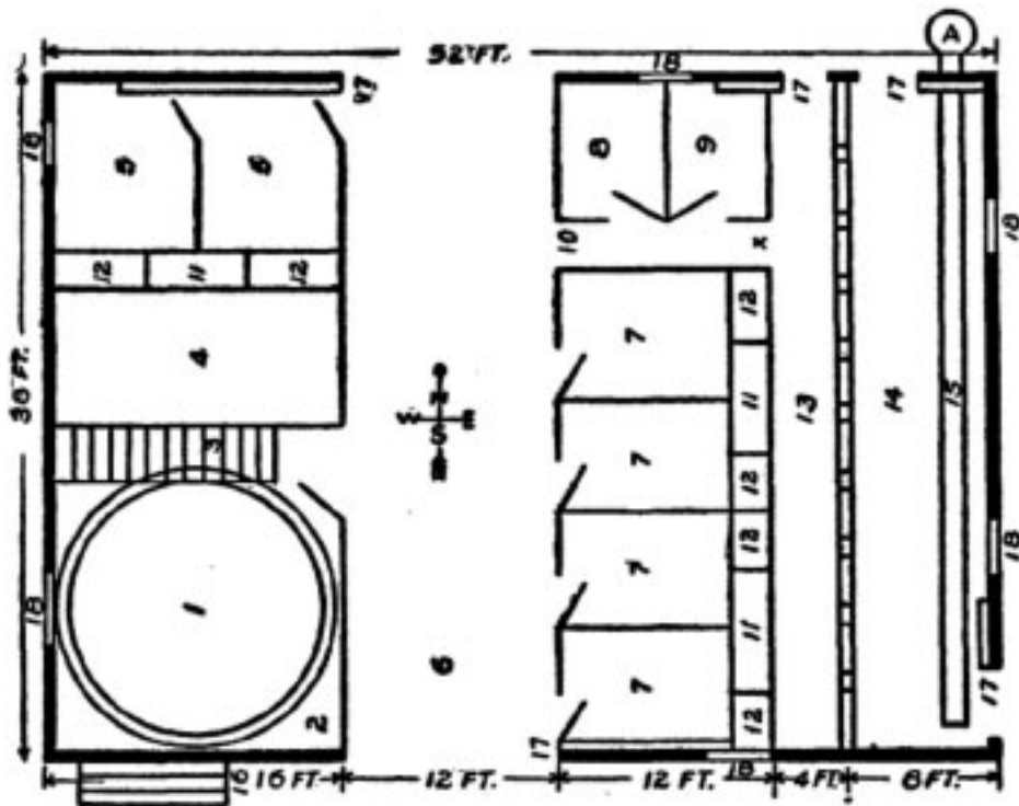
GROUND PLAN OF A KENTUCKY BARN
