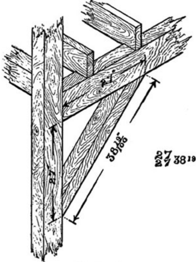
BRACE RULE
