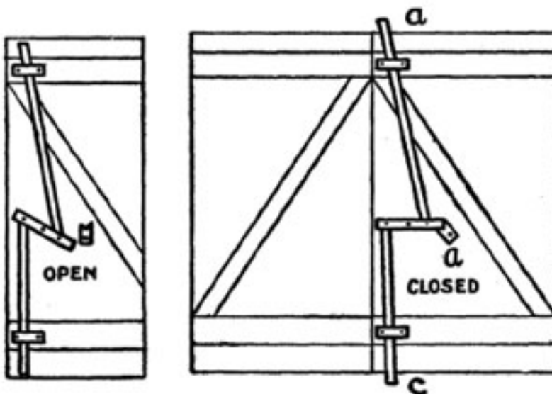
LATCH FOR DOUBLE DOORS
