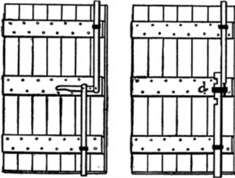
TWO BIG DOOR LOCKS
