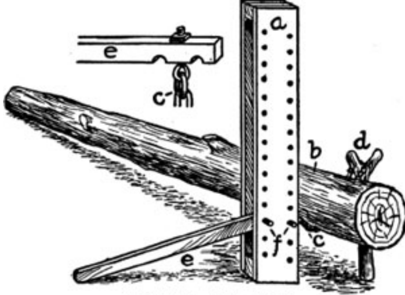
FIGURE 4—LOG JACK
