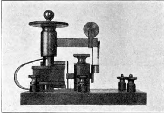
Figur 21. Barretter.
