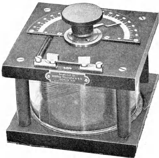
Figur 2. Variabler Kondensator.
