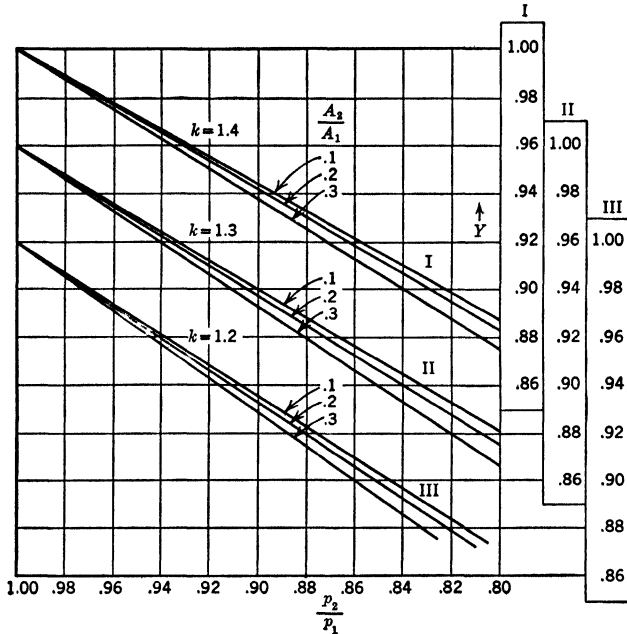
FIG. 160. The Expansion Factor, Y .
