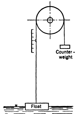
FIG. 143. Float for Measurement of Surface Elevation. (Schematic.)
