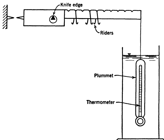
FIG. 130. Westphal Balance.
