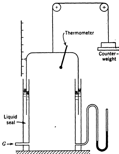
FIG. 158. Gasometer.
