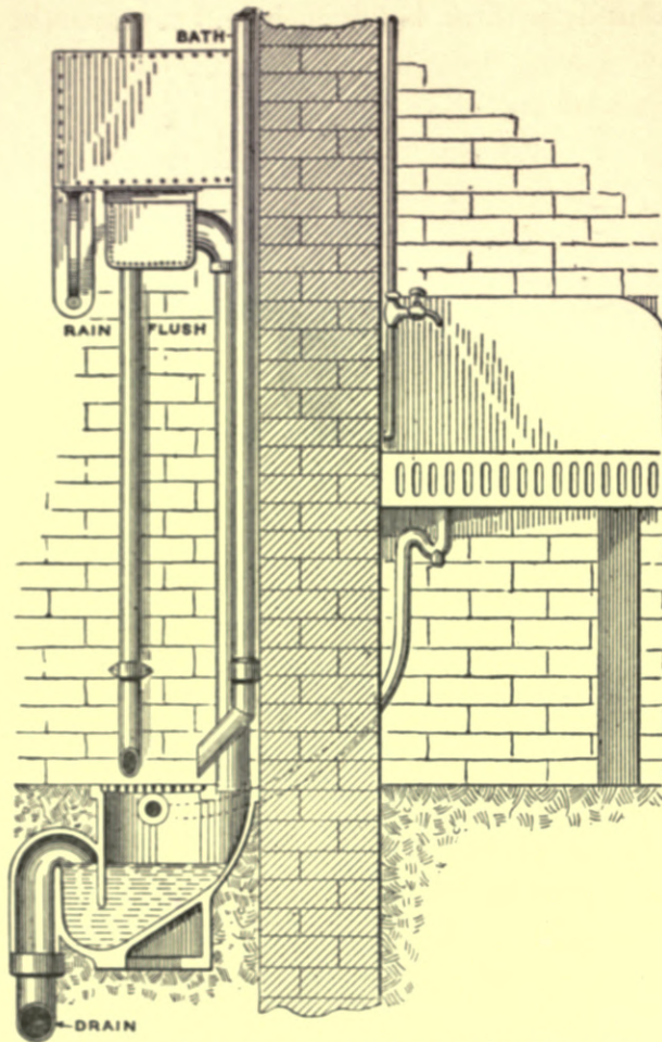
Fig. 392. —Bowes-Scott & Western's Automatic Flushing Grease-trap.
