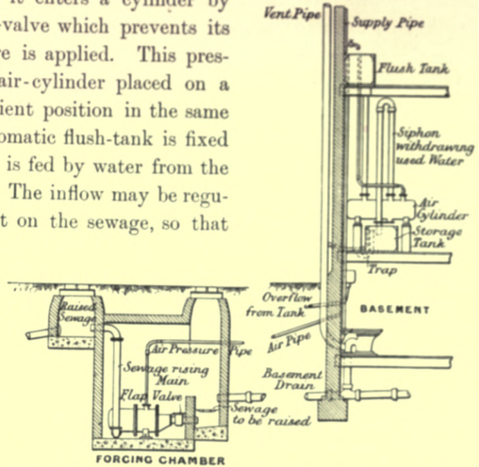
Fig. 363. — Adams's Automatic Sewage-Lift.
