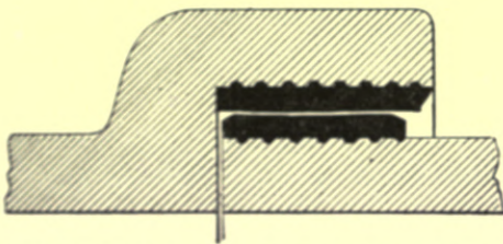
Fig. 321.—Doulton's "Self-adjusting" Drain-pipe Joint.
