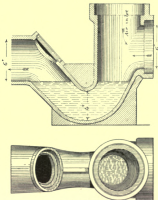
Fig. 367.—Section of the "Cerus" Intercepting Trap.
