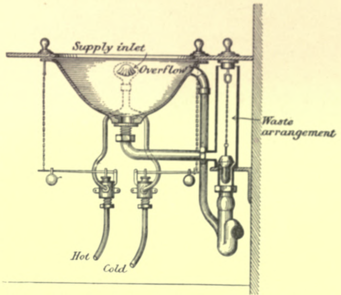
Fig. 269.—Section of Lavatory Basin, showing Waste-valve, Overflow-pipe from Basin to Trap, and Supply-inlet without visible Taps.
