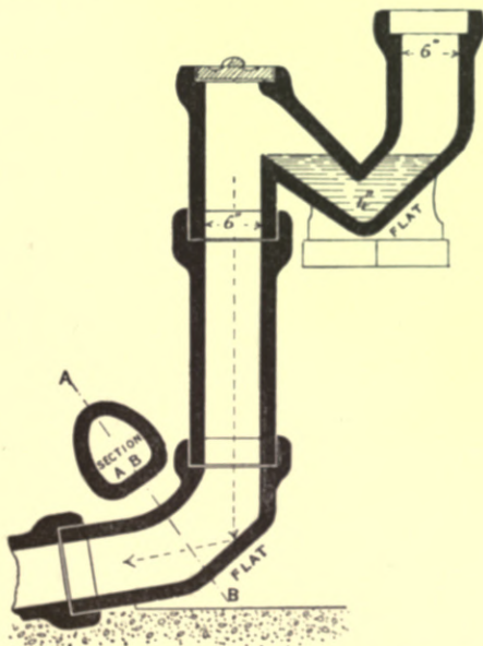
Fig. 373.—Section showing Change of Level by means of "Loco" Trap and Bend.
