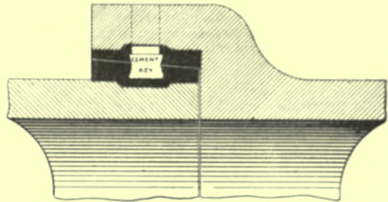
Fig. 324.—Button's "Secure" Joint.
