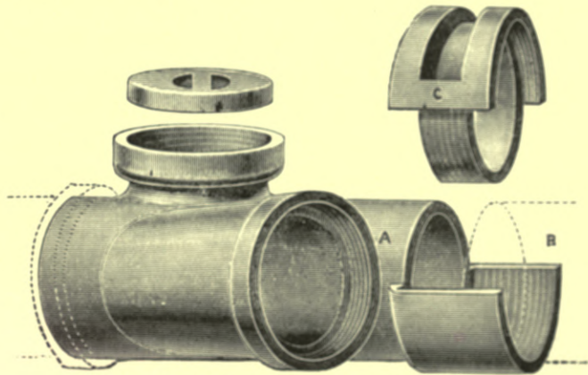
Fig. 399.—Doulton's Patent Junction-pipe.
