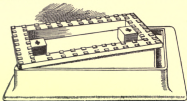
Fig. 347. — Adams's Air-tight Manhole-cover to receive Concrete Filling. 1
