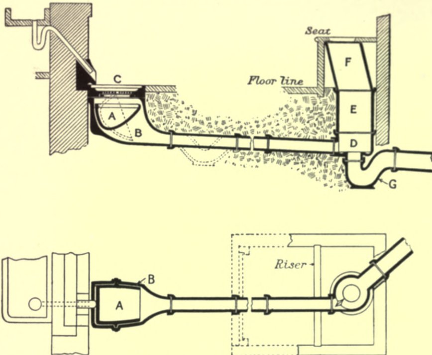
Fig. 289.—Plan and Section of Duckett's Automatic Slop-water Closet.
