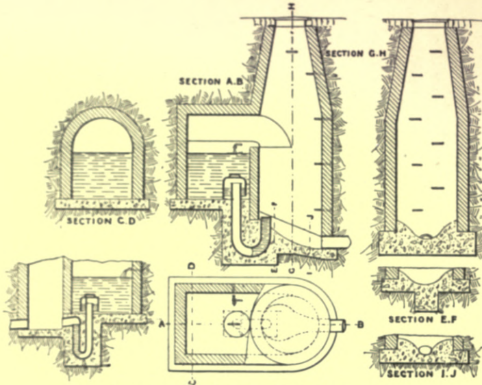
Fig. 413. - Details of the Miller Syphon in Manhole.
