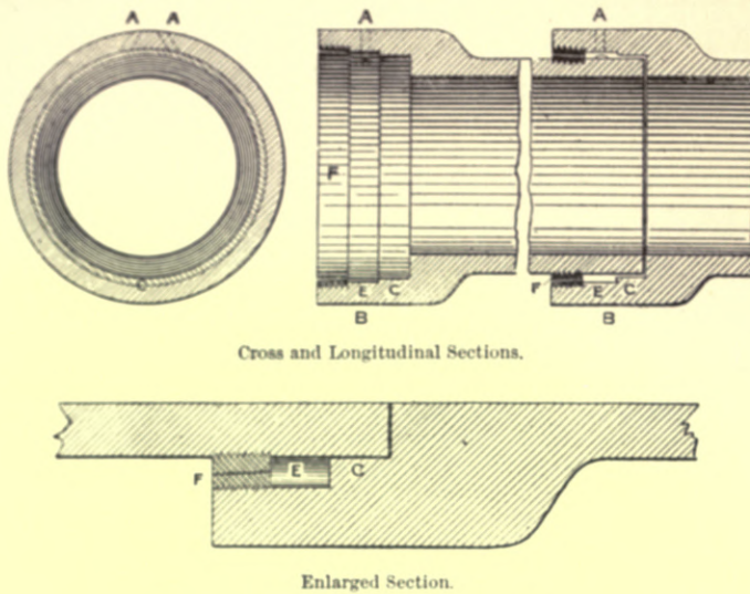
Fig. 325.—Green's "Truinvert" Drain-pipe Joint.
