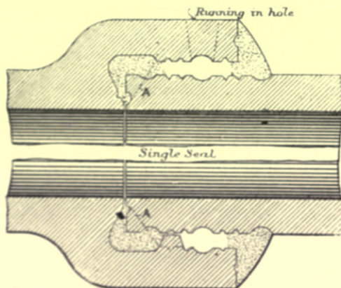
Fig. 326.—Ames and Crosta's Single-seal Drain-pipe Joint.
