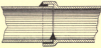
Fig. 316. — Faulty Drain-pipe Joint:— Ridge of Cement.
