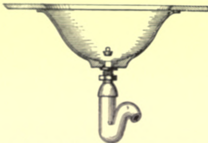
Fig. 206.—Bad Arrangement of Waste from Lavatory Basin—small plug Outlet and large Trap.
