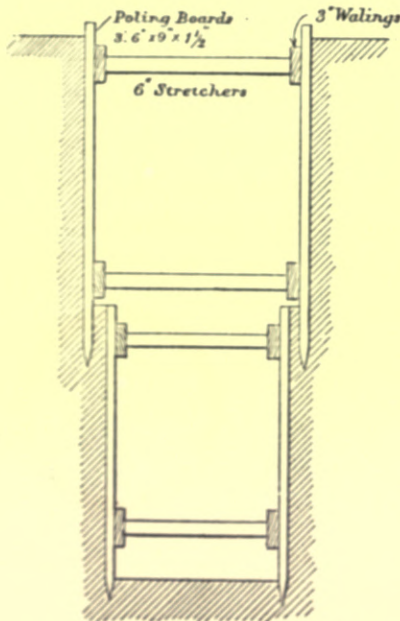
Fig. 403.—Method of Timbering Trench.
