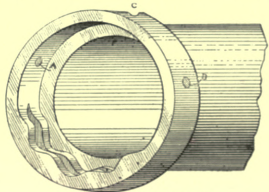
Fig. 328 — Wakefield's Drain-pipe Joint.
