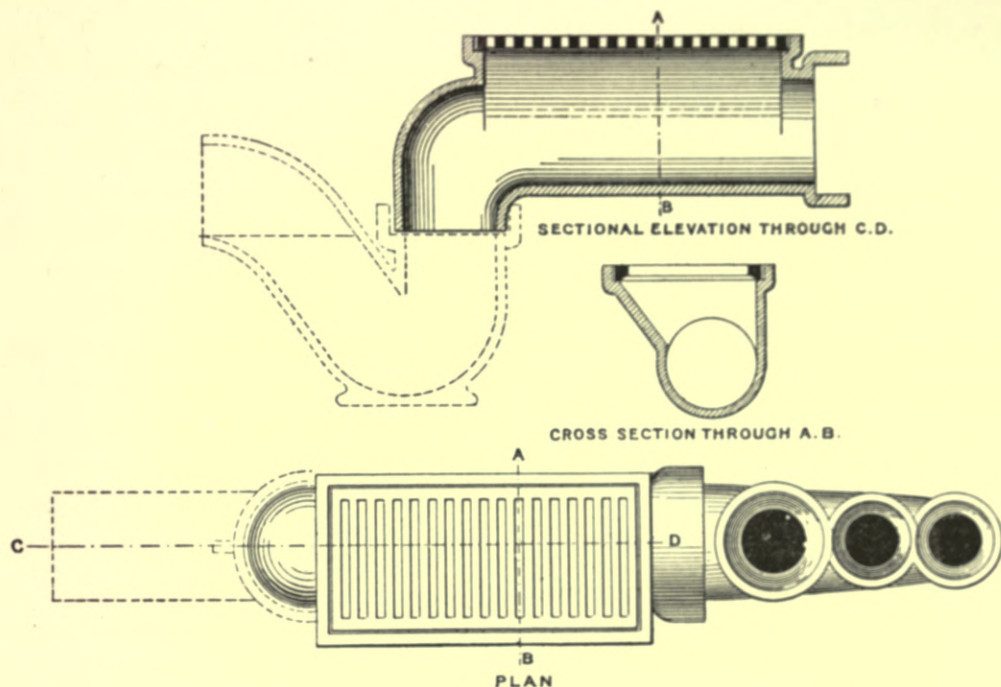
Fig. 383.—Sykes's Slipper, &c., for Waste-pipes.
