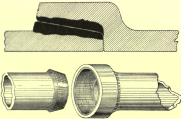
Fig. 320.—Stanford's Drain-pipe Joint.
