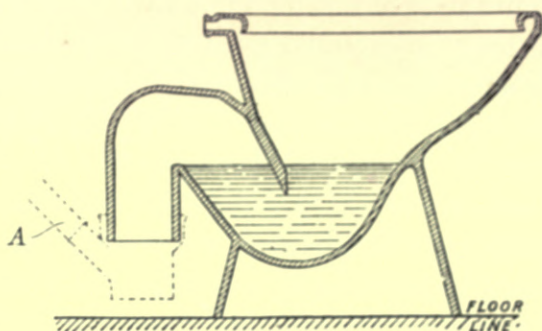
Fig. 293.—Section of Wash-down Pedestal Closet.
