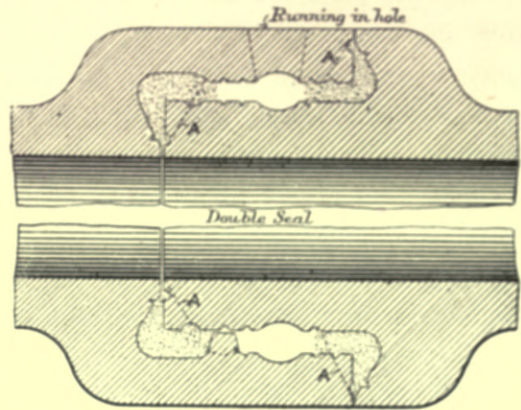
Fig. 327 — Ames & Crosta's Double-seal Drain-pipe Joint.
