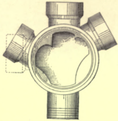
Fig. 350.—Plan of "Tron" Inspection-eye Four-way Junction.
