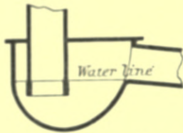
Fig. 286.—Section of "D"-trap.
