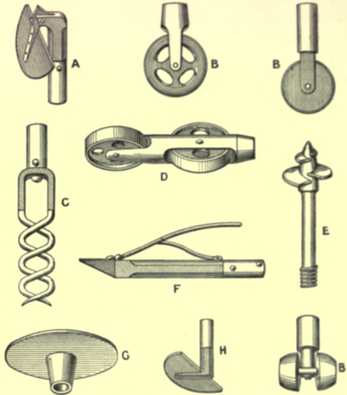
Fig. 417.—Drain-clearing Tools.
