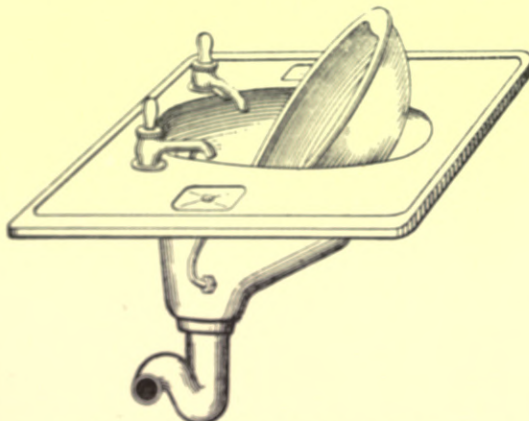
Fig. 272 — "Tip-up" Basin with Receiver and Trap, and with Drainers from Soap-dishes taken into the Receiver.
