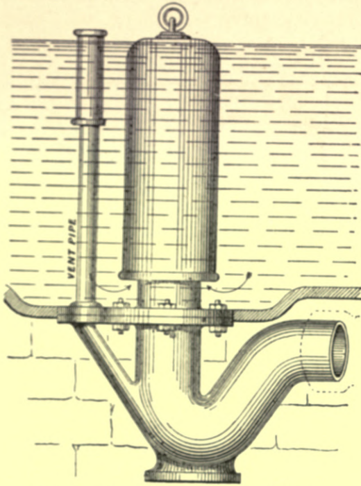
Fig. 410.—Adams's Glazed-ware Flush-tank, for Use with Waste-water.
