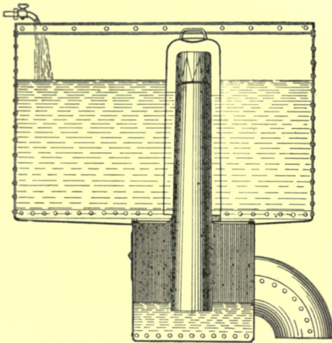
Fig. 405.—Section of Field's Annular Syphon.
