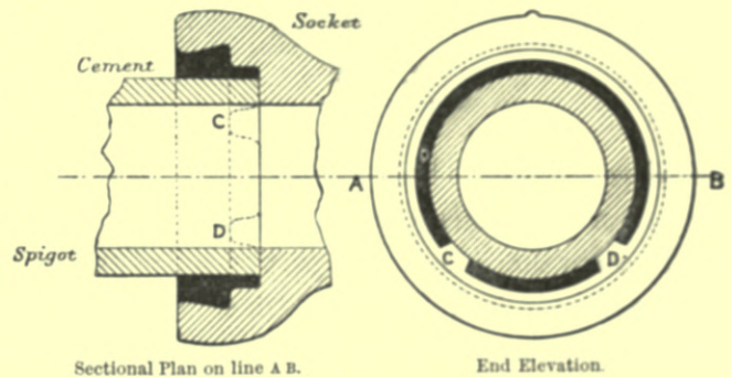
Fig. 319.—The "Loco" Self-centring Joint.
