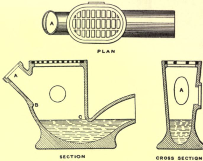
Fig. 390. — Le Rossignol's Self-cleansing Grease-gully.
