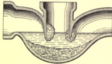
Fig. 365.—Syphon-trap with Hand-hole.
