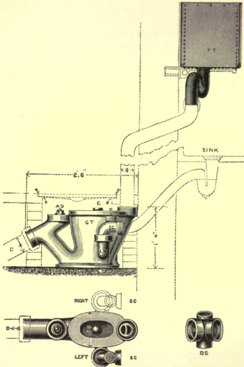
Fig. 391.—Hellyer's Flushing Grease-trap.
