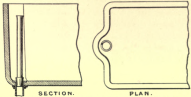
Fig. 264. —Section and Plan of Combined Waste and Overflow inside Bath.
