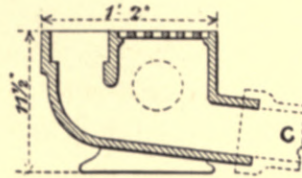
Fig. 352.—Hellyer's Rain-water "Shoe".
