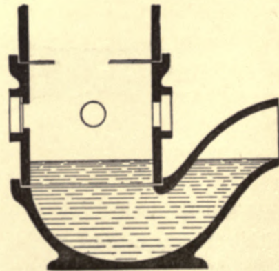
Fig. 394. —Winsor's Flushing-rim Grease-gully with Raising-piece.
