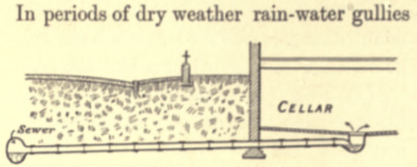
Fig. 354.—Bad Arrangement of Cellar-drainage.
