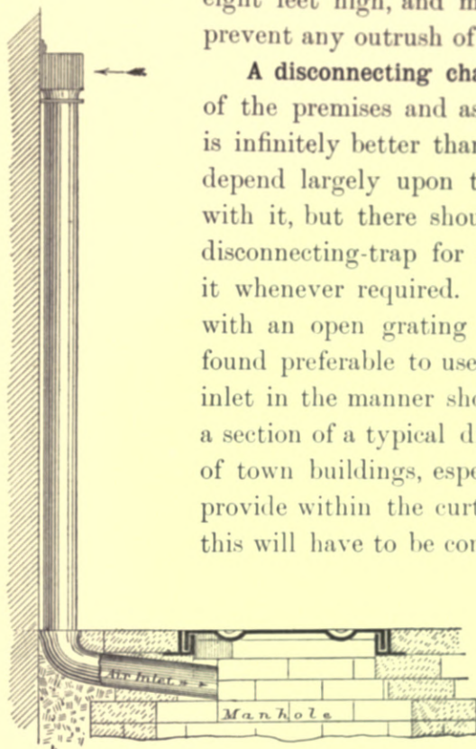
Fig. 334.—Air-inlet to Drain fixed to Wall.
