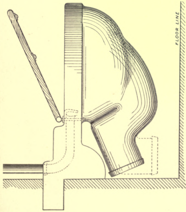
"CORBEL" W.C.
