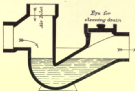
Fig. 366.—Section of the Buchan Intercepting Trap.
