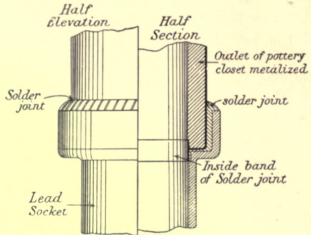
Fig. 297.—Doulton's "Metallo-ceramic" Joint between Earthenware and Lead.
