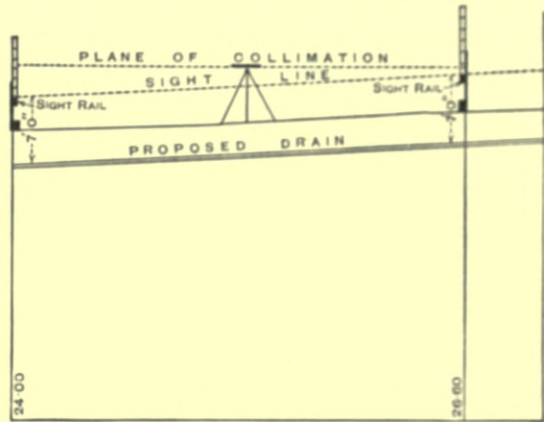
Fig. 397. — Method of Setting up Sight-rails.
