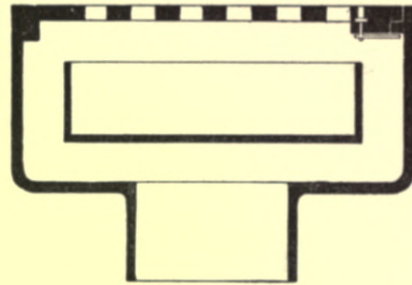
Fig. 333.—Ham Baker & Co.'s Air-inlet Cover.
