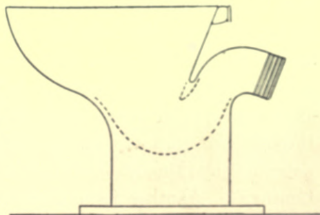
Fig. 294.—Elevation of the "Kenon" Pedestal Wash-down Closet.
