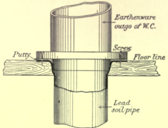
Fig. 299.—Flange Joint—screwed to Floor.
