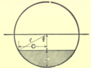
Fig. 311.—Diagram to illustrate Trigonometrical Calculation of the Discharge from a Circular Drain.
