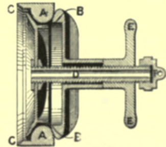
Fig. 422.—The "Addison" Drain-stopper.
