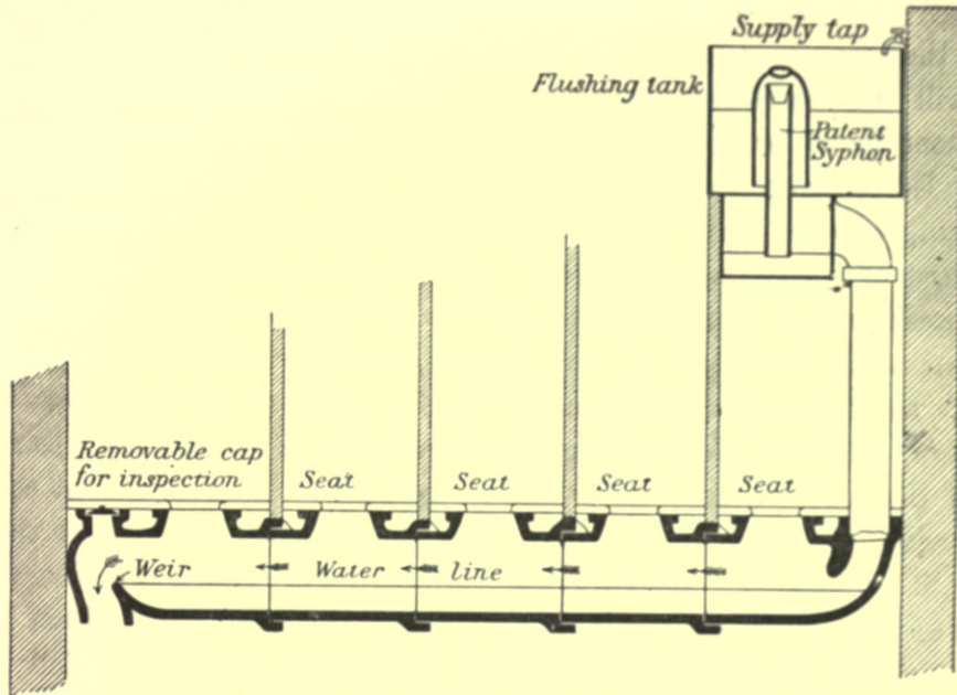
Fig. 291.—Section of Trough-closet with Automatic Flushing Tank.
