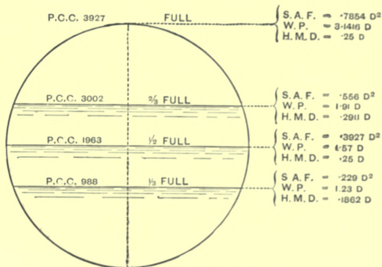
Fig. 310 — Data for Calculating Flow in Circular Sewers.
