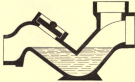
Fig. 369.—Section of Stidder's Drop Trap.
