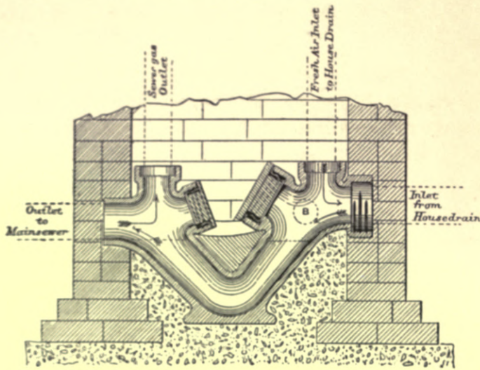
Fig. 378.—Section of Sykes's Interceptor in Manhole.
