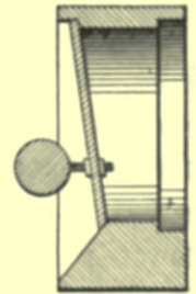
Fig. 358. — View and Section of Balance Flap-valve.
