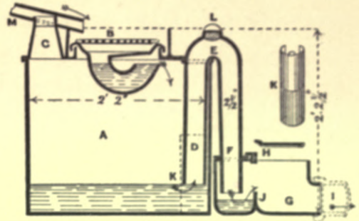
Fig. 408.—Section of Field's Self-acting Flush-tank.
