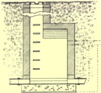
Fig. 339 — Vertical Sections of Deep Manhole.
