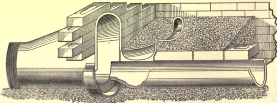
Fig. 416.—Drain Shoot for Use with Penstock.
