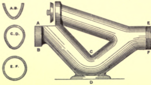
Fig. 375.—Improved "Kenon" Intercepting Trap.
