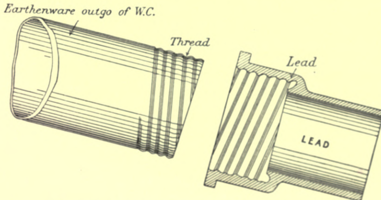
Fig. 300.—Freeman's Screw Connection between Earthenware and Lead.
