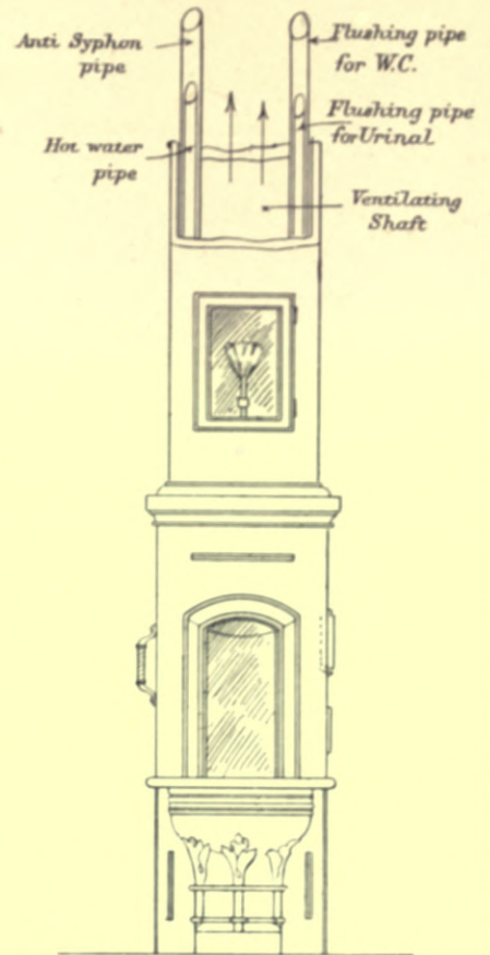
FRONT ELEVATION (to a smaller scale).
