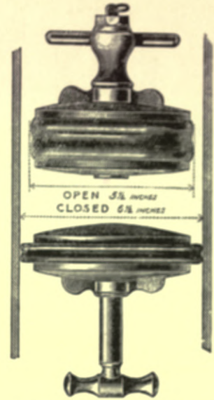
Fig. 420.—Jones's Screw Expanding Pipe stopper.
