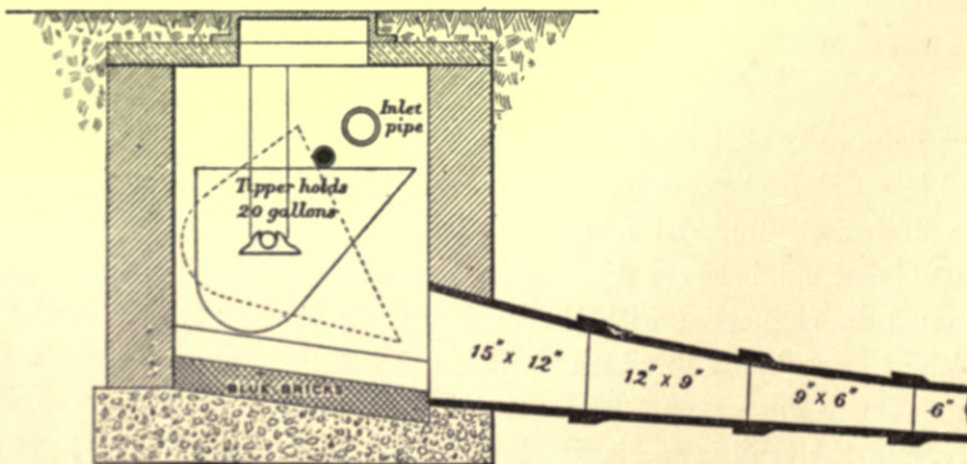
Fig. 411.—Duckett's Tipper used for Flushing Drains.
