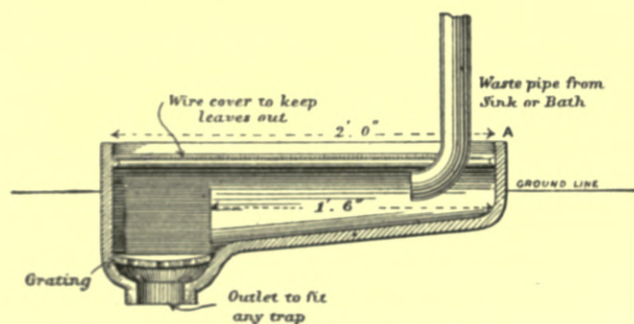
Fig. 381.—Docking's Channel for Waste-pipes.
