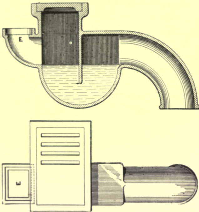
Fig. 353.—Spinks's Cast-iron Rain-water Disconnecting Gully.
