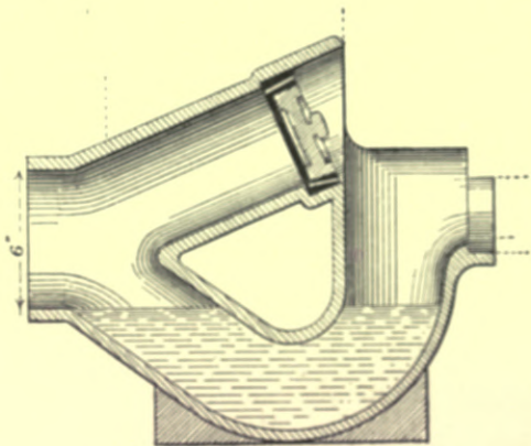
Fig. 374.—Section of "Beancliff" Intercepting Trap for Manhole.
