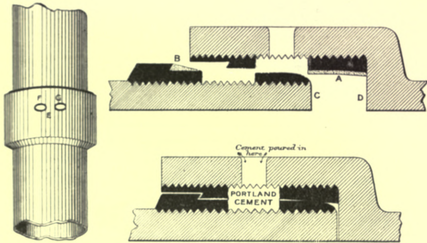
Fig. 323.—Hassall's Double-lined Drain-pipe Joint.
