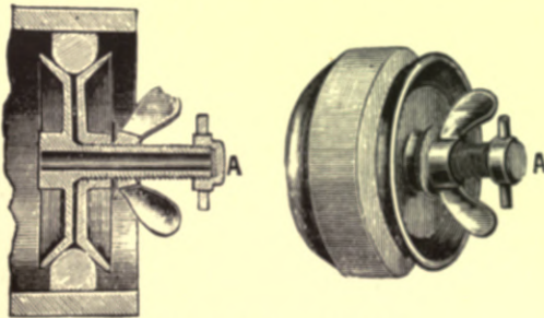
Fig. 421.—Syer's "Grip" Plug.
