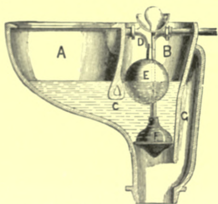
Fig. 288.—Section of the Twin-basin Closet.
