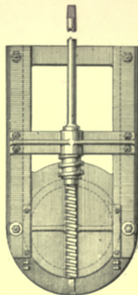
Fig. 414.—Screw-down Penstock.
