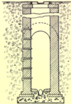
Fig. 339 — Vertical Sections of Deep Manhole.
