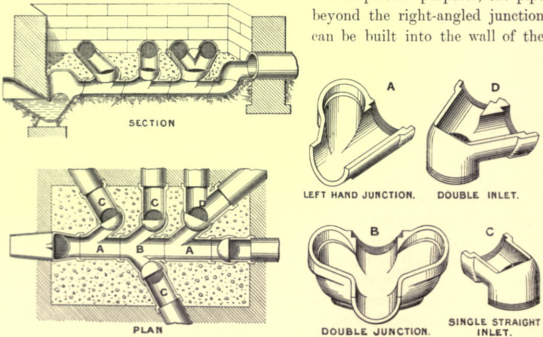
Fig. 344.—Wyvurst Channel-bends.
