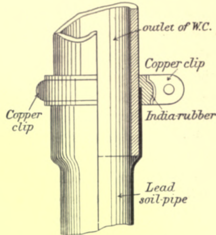
Fig. 302.—Humpherson's Joint.
