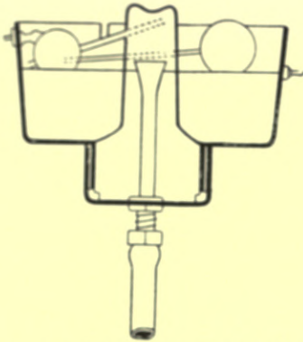
Fig. 304 — Section of Bean's Direct-acting Valveless Waste-preventer.
