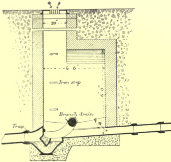
Fig. 335.—Section of Intercepting Chamber with Air-Inlet Cover.
