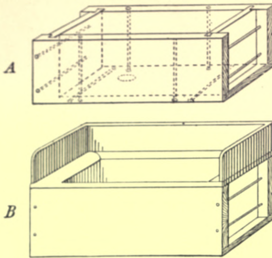
Fig. 277.—Wood Sink for Washing Silver, &c. A, the Framework; B, the completed Sink.
