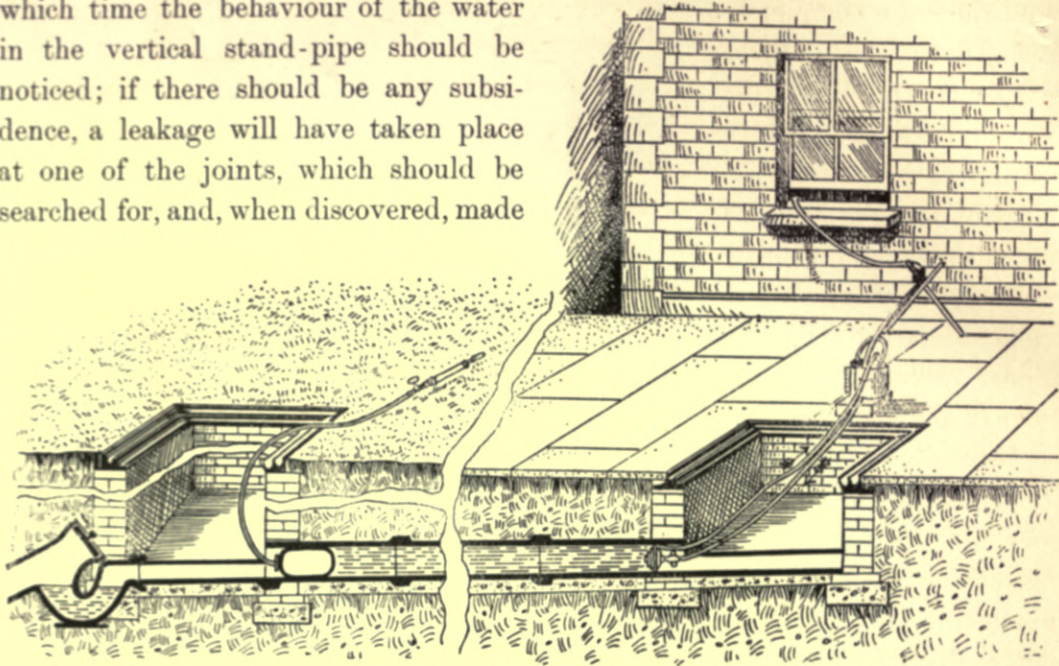
Fig. 418.—Jones's Apparatus for Testing Drains with Water.
