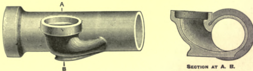
Fig. 401.—Codling's Patent Rest-Bend Junction.
