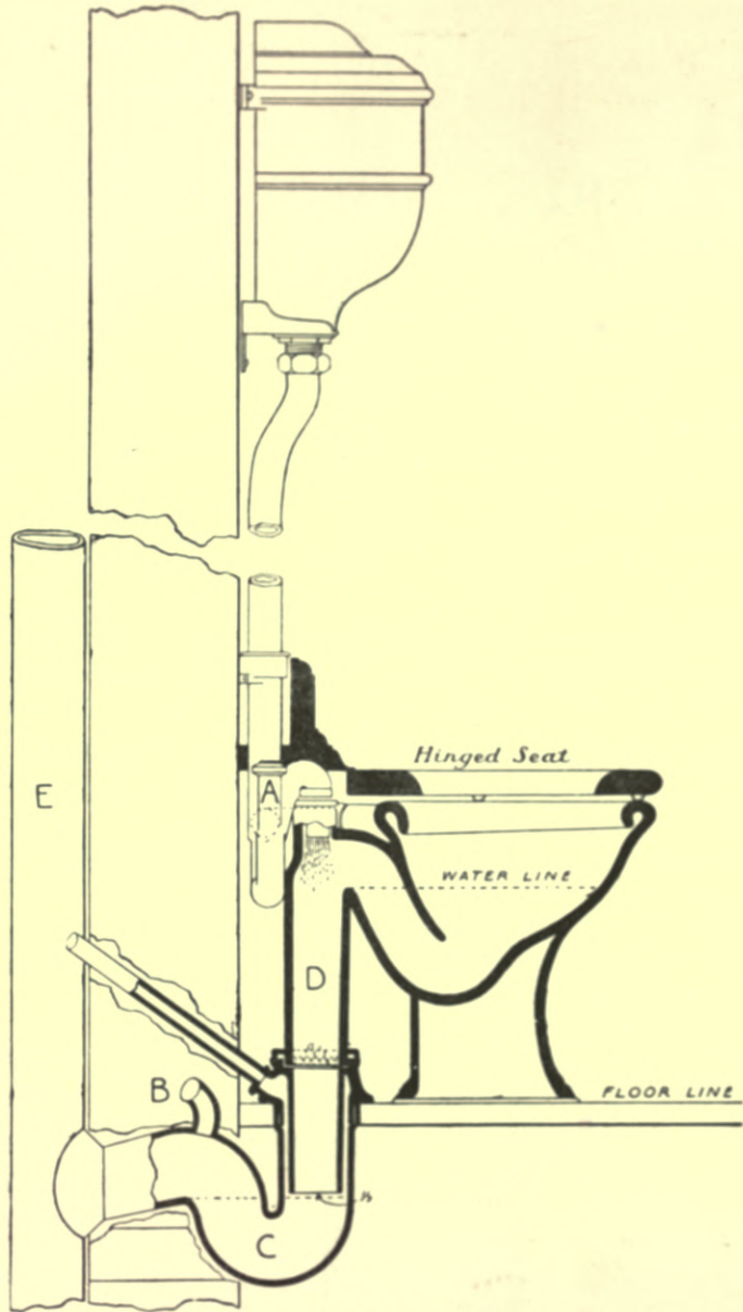
Fig. 295.—Jennings & Morley's Syphonic Water-closet.
