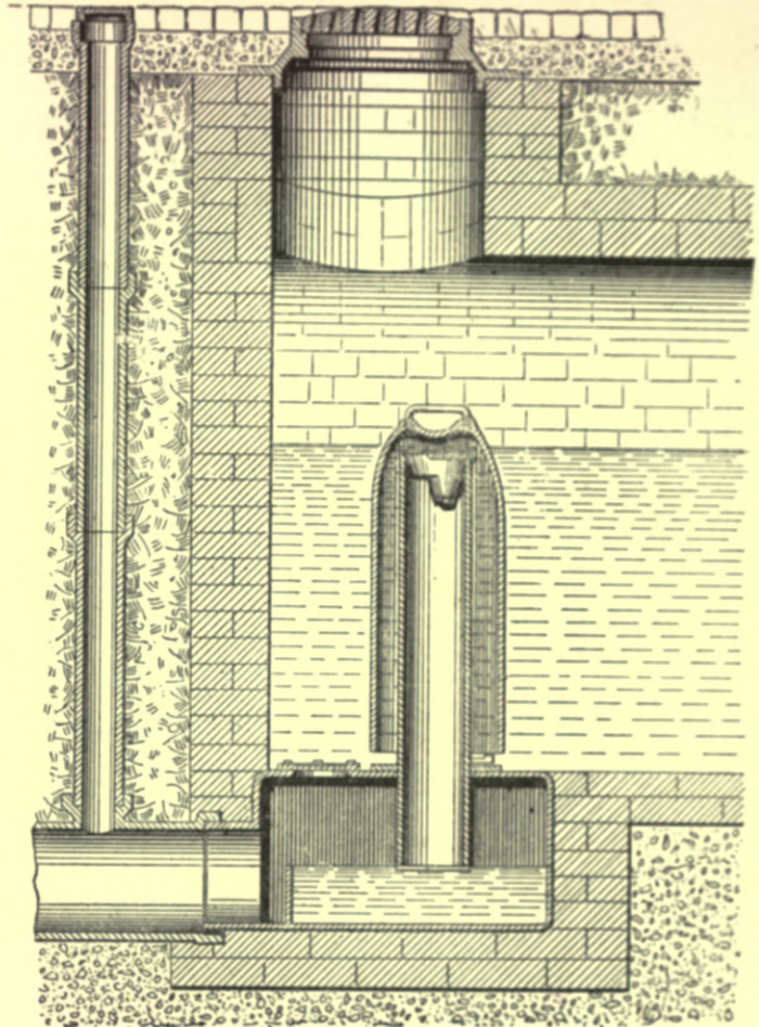
Fig. 412.—Field's Automatic Flushing Syphon in Brick Tank.
