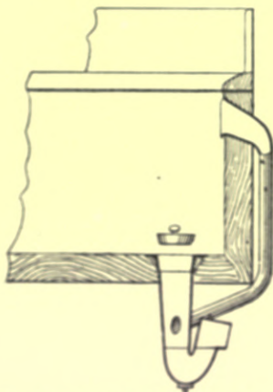
Fig. 278.—Plug-waste and Overflow from Wood Sink.
