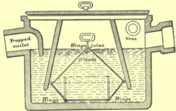
Fig. 388.—"Eclipse" Grease-trap.
