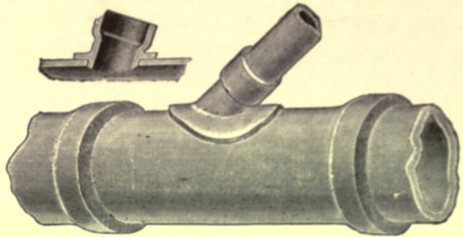
Fig. 398.—Section and Plan of Saddle-junction for Branch-drain.
