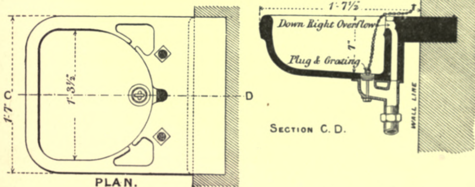
Fig. 267.—Hellyer's Fire-clay "Corbel" Lavatory Basin, with "Downright" Overflow.
