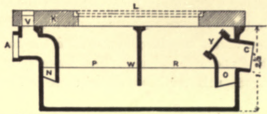
Fig. 387.—Hellyer's Stoneware Grease-gully, for Large Houses, Hotels, &c.
