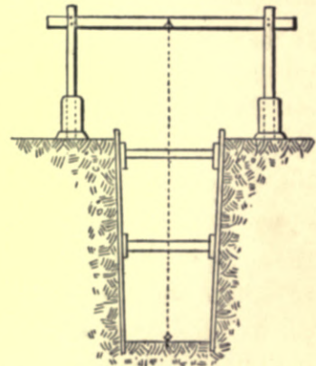
Fig. 396.—Sight-rail for Laying Drains.
