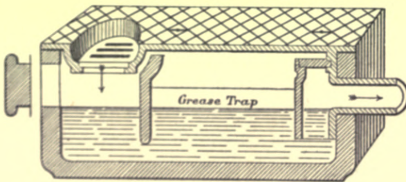
Fig. 386. — Adams's Grease-trap.
