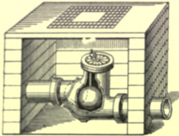
Fig. 361. — Dyer's Valve for preventing Back-water.
