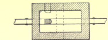
Fig. 340.—Section and Plan of Shallow Manhole.
