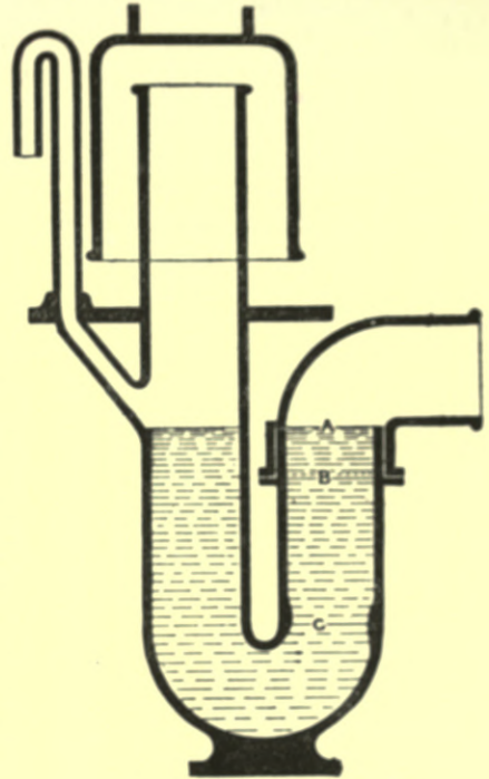
Fig. 406.—Section of Adams's Flushing Syphon.
