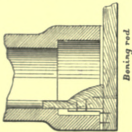
Fig. 395.—Shoe for Boning-rod.
