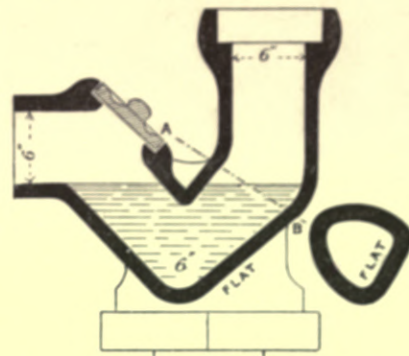
Fig. 372.—Section of "Loco" Intercepting Trap.
