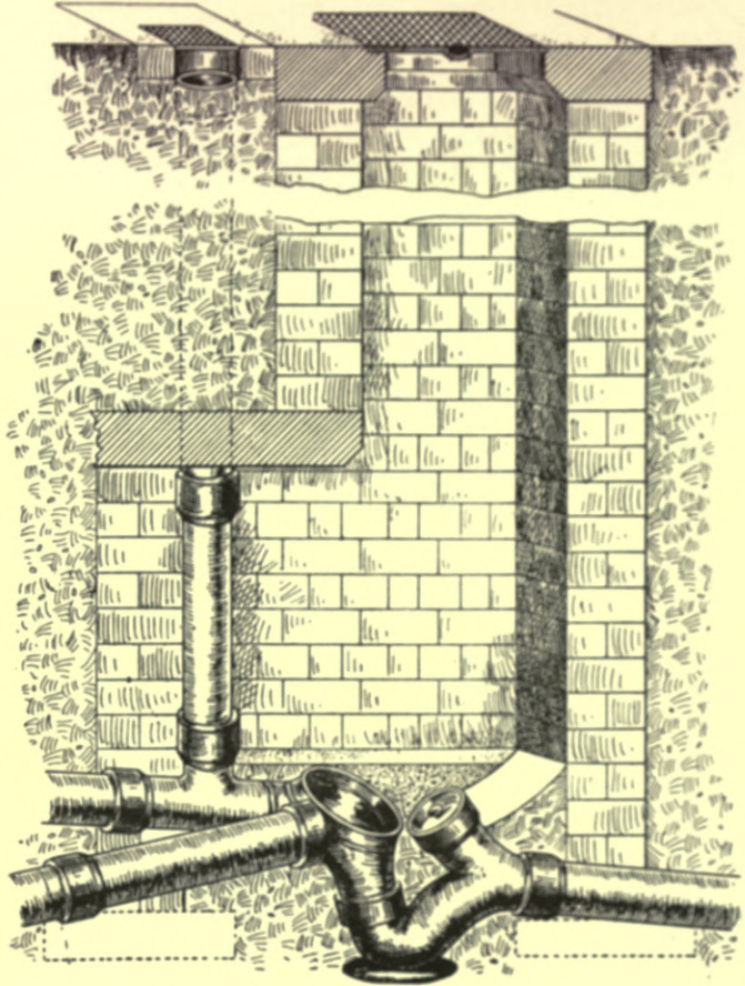
Fig. 377.—"Waverley" Closed Intercepting Trap fixed in Manhole.
