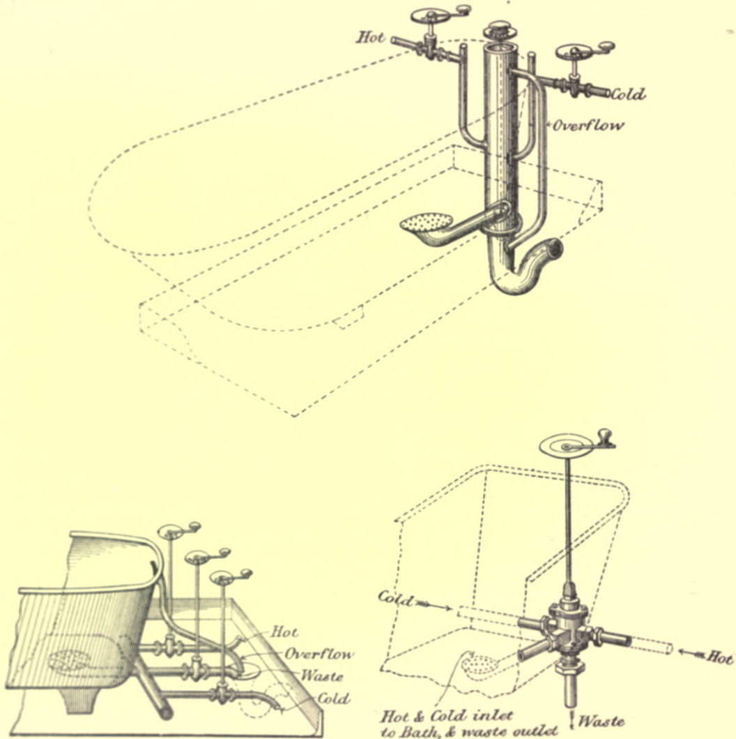
Figs. 257, 258, 259.—Three Bad Forms of Bath-supplies and Waste.
