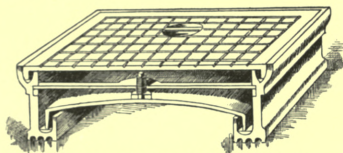
Fig. 348. — Section of Jones's Air-tight Double-seal Manhole-cover.
