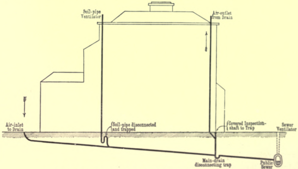
Fig. 331. —Section showing Drain-ventilation with Inlet at Head of Drain.
