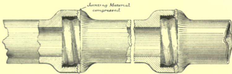
Fig. 329.—Sykes's Patent Drain pipe Joint.
