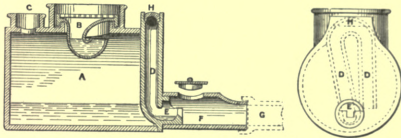
Fig. 409.—Section and End Elevation of Field's Stoneware Flush-tank.
