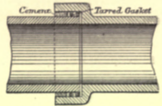
Fig. 318.—Drain-pipe Joint made with Gasket and Cement.
