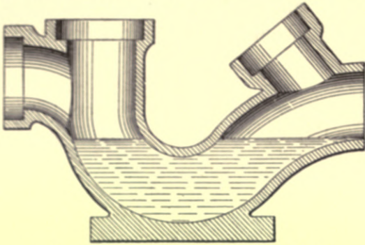
Fig. 368.—Section of Oates and Green's Intercepting Trap.
