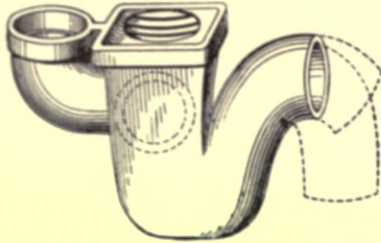
Fig. 351.—Cliff's Rain water Intercepting Gully
