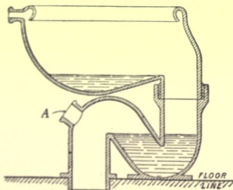
Fig. 292.—Section of Wash-out Closet.
