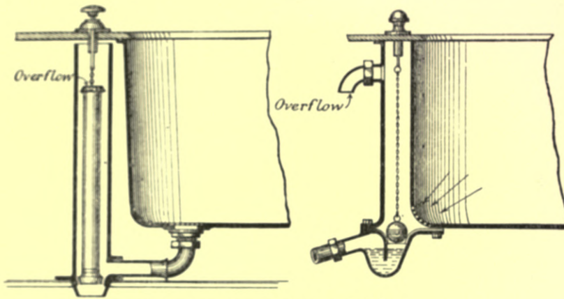
Fig. 262.—Combined Waste and Overflow outside Bath.
