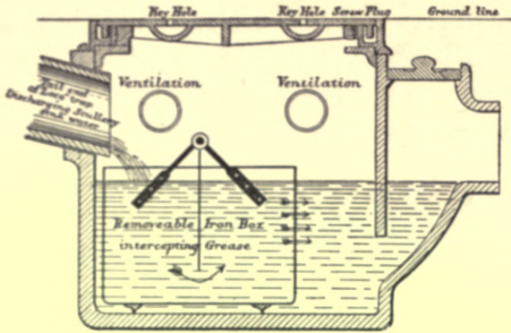
Fig. 384. — "Loco" Grease-trap with Retainer.
