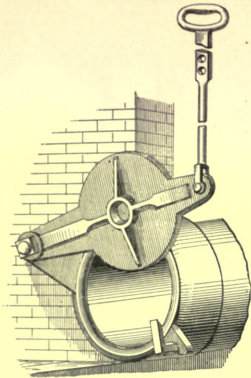
Fig. 415.—Disc Penstock.
