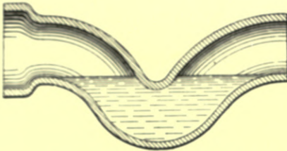
Fig. 364.—Section of Syphon-trap.
