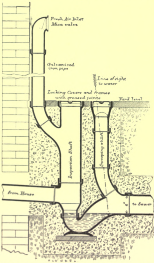
Fig. 370.—Section of Winsor's Villa Detector Trap, with Shafts for Sweeping and Air-inlet, &c.
