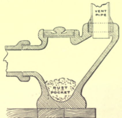
Fig. 338.—"Loco" Rust-chamber at Foot of Ventilation-pipe.
