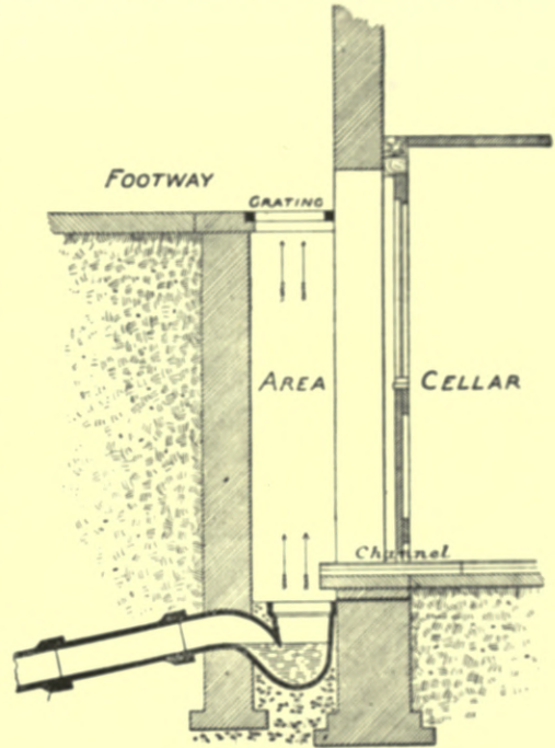
Fig. 354.—Bad Arrangement of Cellar-drainage.
