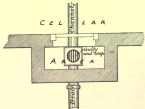
Fig. 355.—Plan and Section of Area, &c., for Cellar-drainage.
