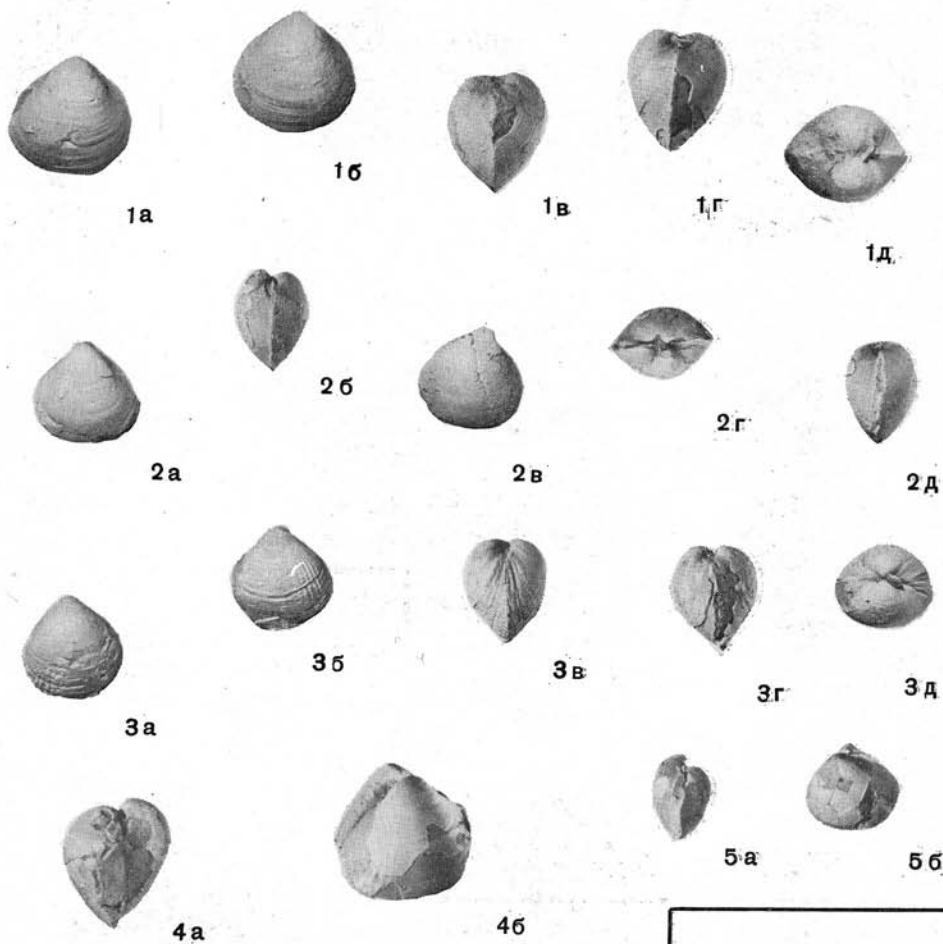
Protocardia concinna
