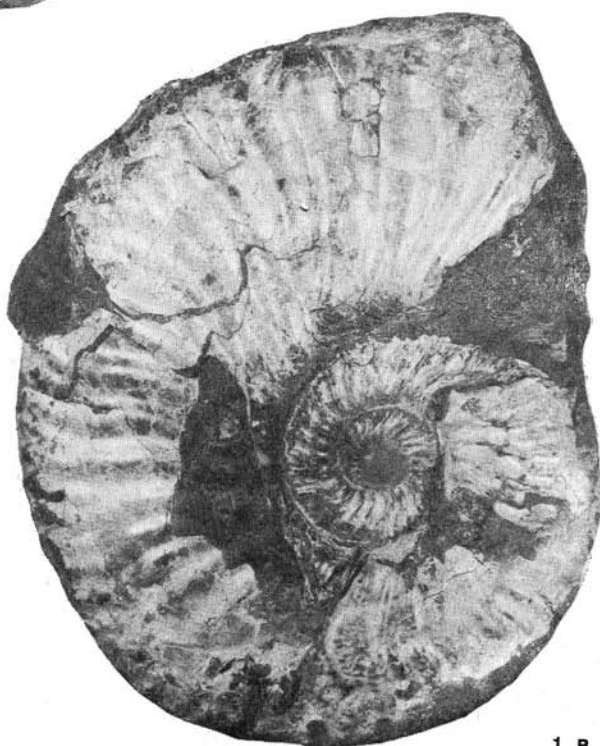
Deshayesites collevarus
