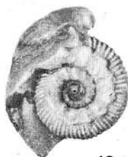
Simbirskites umbonatus
