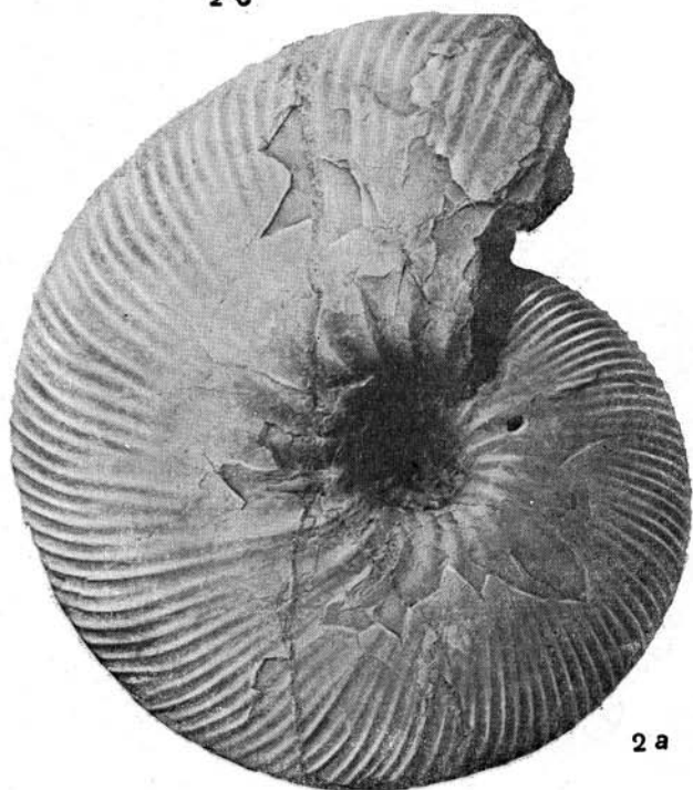
Craspedodiscus discofalcatus
