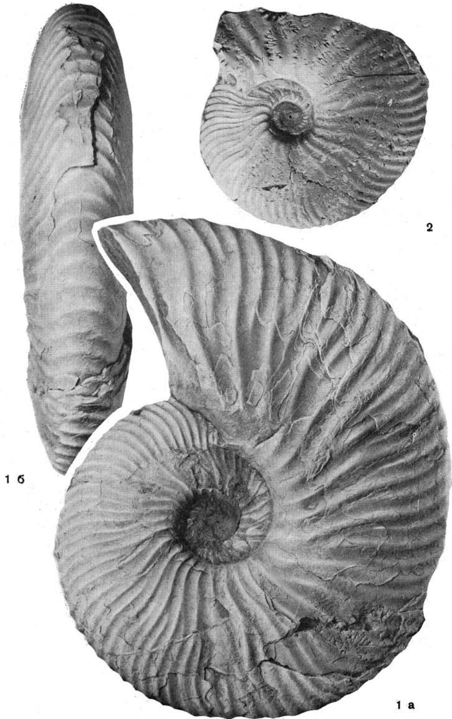
Deshayesites imitator
