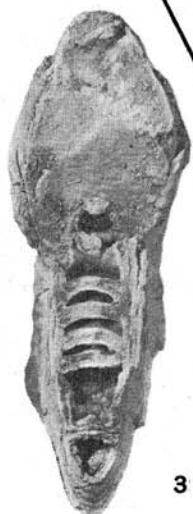
Deshayesites variabilis
