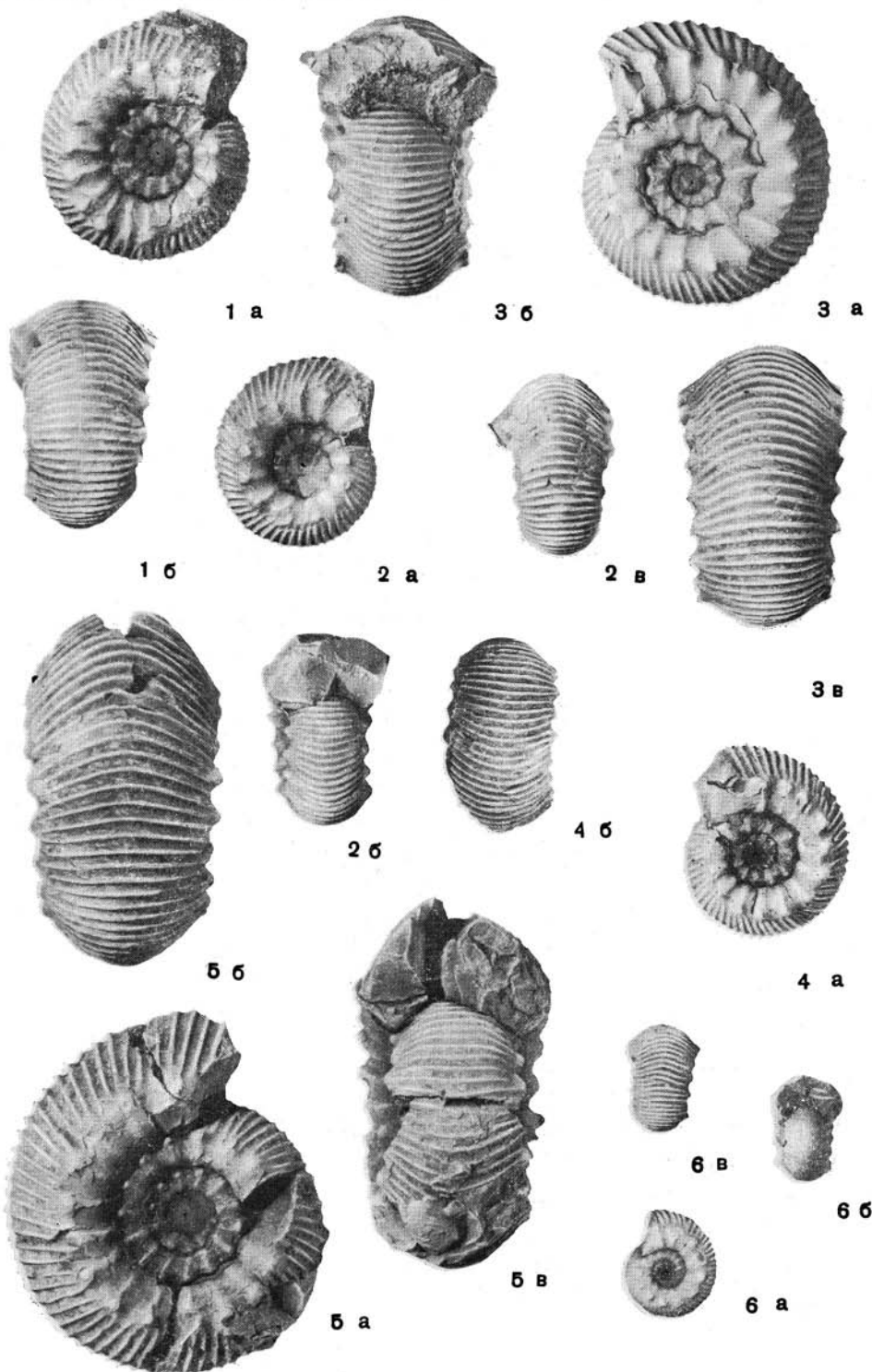
Simbirskites umbonatus
