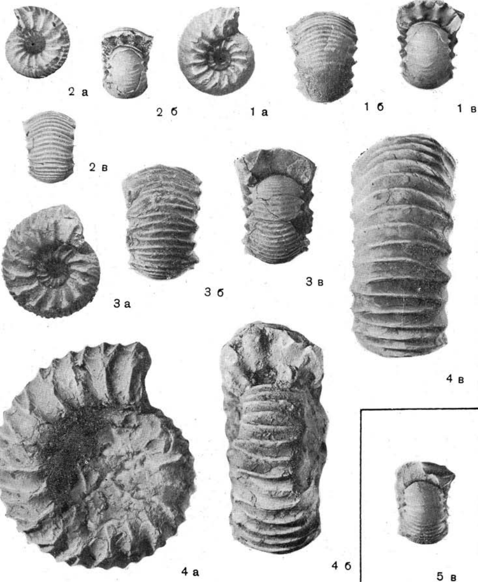
Speetoniceras pavlovae
