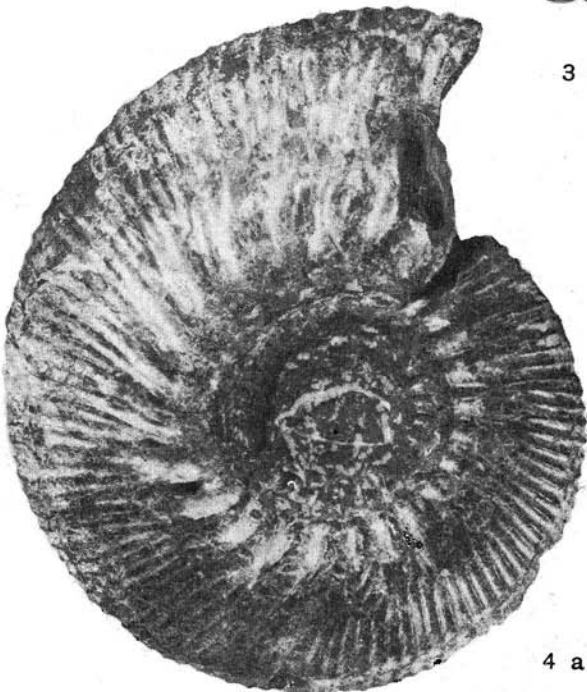
Simbirskites pseudobarboti
