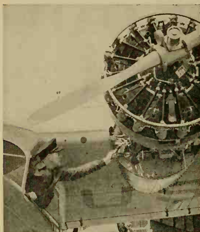
FIG. 153. Starting an airplane engine by means of a cartridge. (Photograph by Rudy Arnold.)
