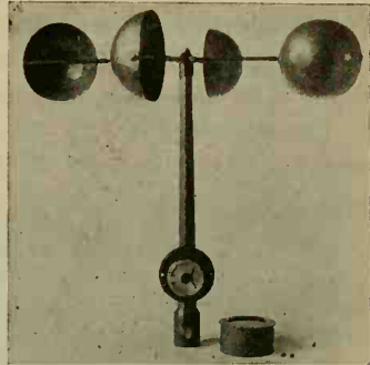
FIG. 84. Robinson four-cup anemometer with cups attached and dial cover off. (Courtesy of the U. S. Weather Bureau.)
