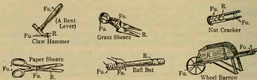
FIG. 103. To which class does each of these everyday levers belong? (From Pieper and Beauchamp's Everyday Problems in Science , published by Scott, Foresman and Company.)
