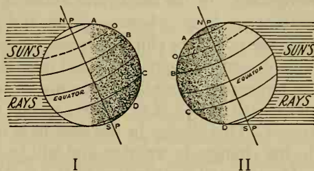
FIG. 76. I, the earth in June; II, the earth in December. (From the Yerkes Observatory, reprinted by permission of the Chicago University Press.)
