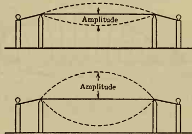
FIG. 217. Intensity depends upon amplitude
