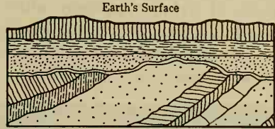
FIG. 51. An unconformity.
