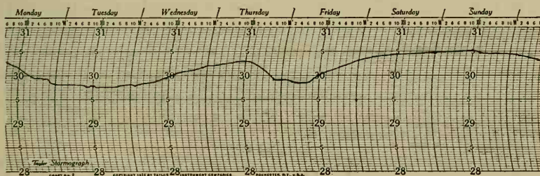
FIG. 87B. An atmospheric pressure record for the week, January 11-17, 1932, at Stockton, California. The weather was stormy during this week.
