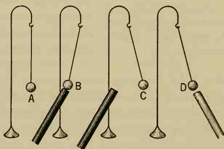
FIG. 228. The hard-rubber rod attracts a pith ball in B, but upon touching it, repels it as shown in C. The pith ball repelled by the rubber rod is attracted by a glass rod that has been charged by rubbing it with silk as shown in D.
