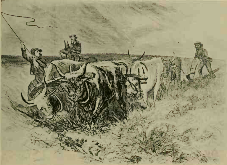
FIG. 59. Plowing on the prairies beyond the Mississippi. (Sketched by Theodore R. Davis.) Six strong oxen were required to pull this plow which is turning over the thick virgin sod of the Great Plains. The pioneer's plow destroyed the luxuriant tall grasses of the Great Plains where the buffalo grazed. (Culver Service, New York.)
