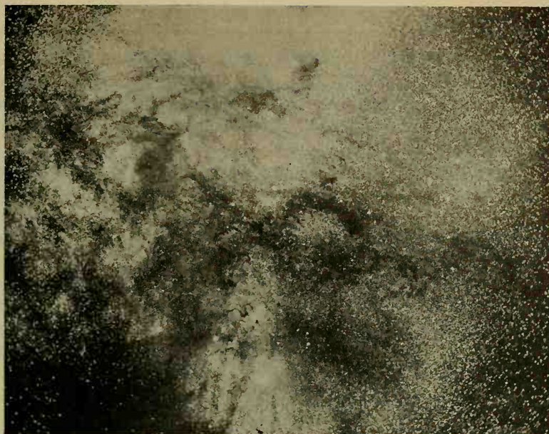
FIG. 7. Milky Way north of Theta Ophiuchi. (Photograph from the Yerkes Observatory, reprinted by permission of the Chicago University Press.)
