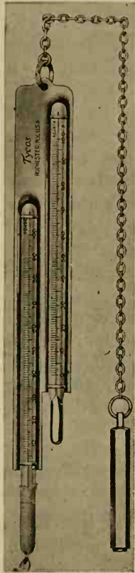
FIG. 78. A sling psychrometer. (Courtesy of Tycoos, Rochester, N. Y.)
