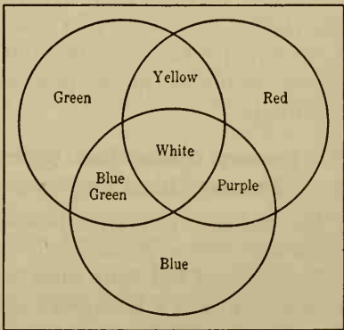
FIG. 184. Mixing additive colors.
