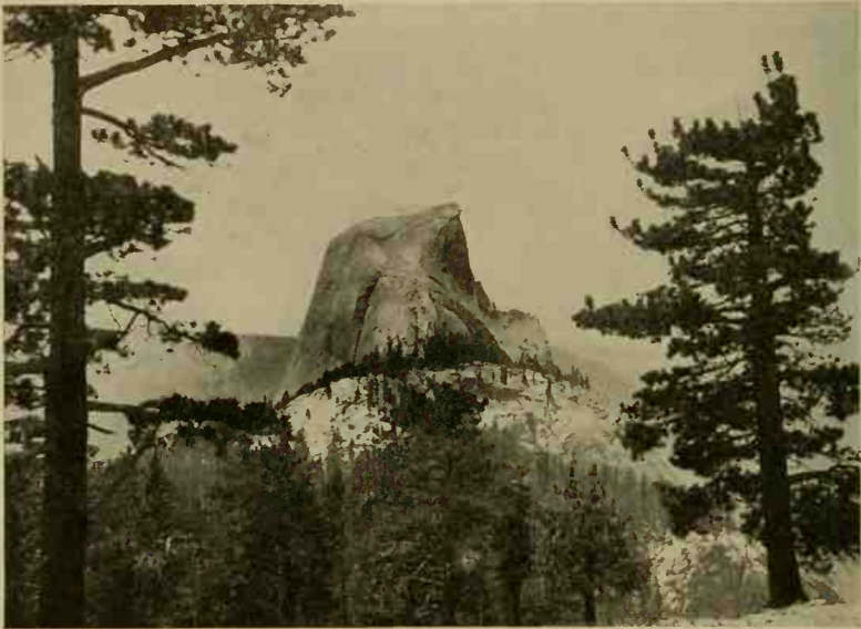
FIG. 37. Half Dome in Yosemite National Park, an example of exfoliation. (Courtesy of the U. S. Geol. Survey.)
