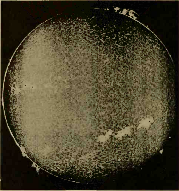
FIG. 20. The sun, showing unusual activity in both focculi and prominences. (Photograph from the Yerkes Observatory, reprinted by permission of the University of Chicago Press).
