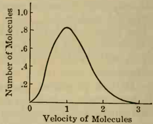
FIG. 73B. The theory of probability shows that molecules subject to chance collisions may be divided into groups, each one with a different range of velocity.
