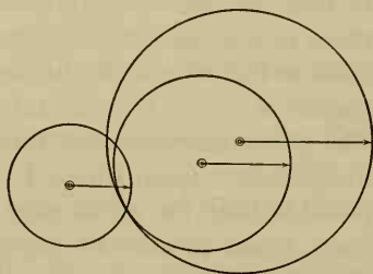
FIG. 44. Three observatories cooperate in locating an earthquake. A circle is drawn around each station as a center, with a radius equal to the estimated distance to the earthquake. The intersection of the three circles is the desired location.
