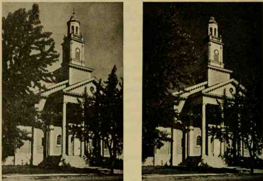
FIG. 191. Left, without Pola screen. Right, Pola screen darkens the sky because the light from the direction at right angles to the sun is partially polarized. (Courtesy of The Polaroid Corporation.)
