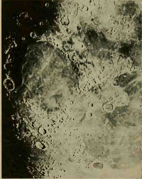
FIG. 24. The Caucasus and Apennine mountains on the moon at eighteen days. (Photograph from the Yerkes Observatory, reprinted by permission of the Chicago University Press.)
