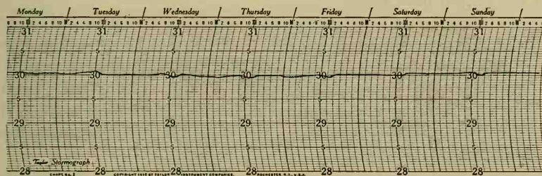
FIG. 87A. An atmospheric pressure record for the week, June 6-12, 1932, at Stockton, California. The weather was fair all week.
