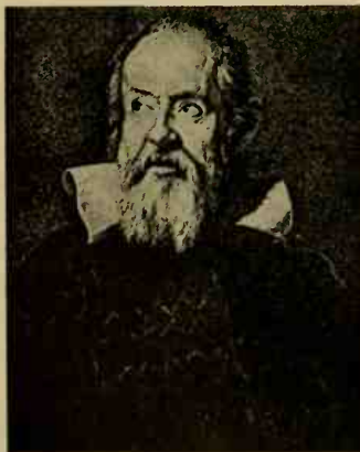
FIG. 2. Galileo. (From the Yerkes Observatory, reprinted by permission of the Chicago University Press.)
