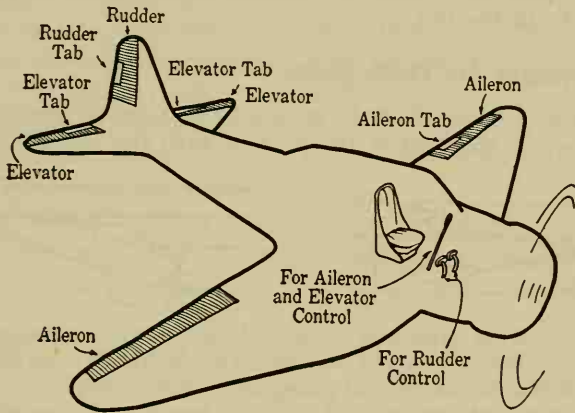
FIG. 165. How an airplane is controlled in flight.
