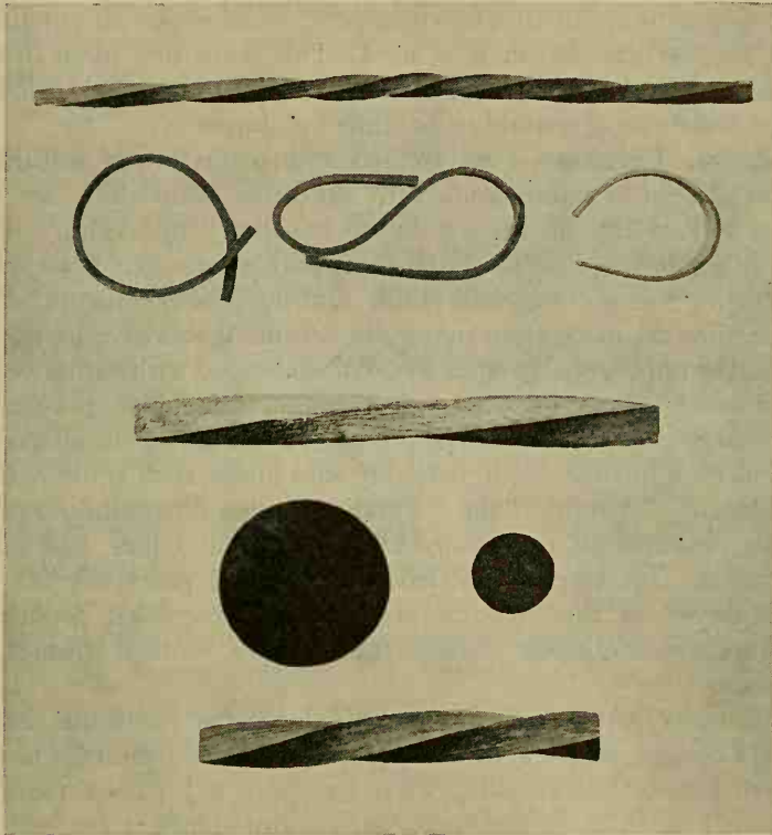
FIG. 289. Wood may be twisted or bent after urea treatment. (Courtesy of the U. S. Forest Products Laboratory.)
