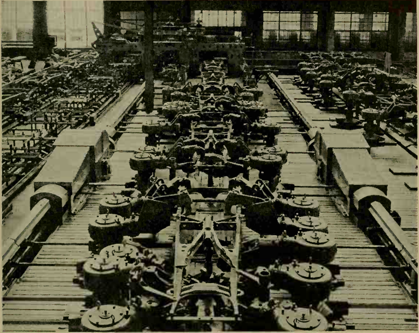
FIG. 108. Automatic automobile frame plant. Capacity of automatic plant, 8000 finished and painted frames per day. (Courtesy of the A. O. Smith Corporation.)
