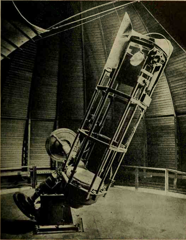
FIG. 5. The 24-inch reflecting telescope of the Yerkes Observatory. (An astronomical photograph from the Yerkes Observatory, reprinted by permission of the Chicago University Press.)
