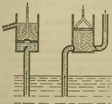
FIG. 67. The lift pump (left) and the exhaust pump (right).
