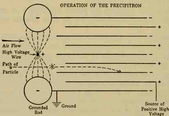
FIG. 96. The principle of the precipitron.
