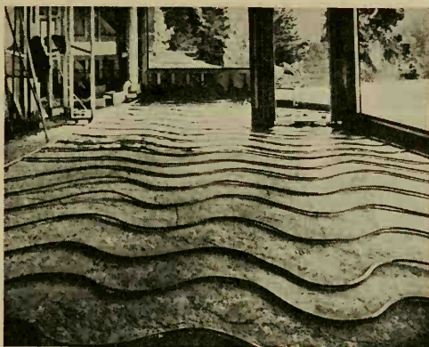
FIG. 97. A floor-warming pipe installation before laying the floor. (Courtesy of the Copper and Brass Research Association.)
