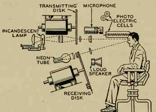
FIG. 265. A two-way telephoto system shown diagrammatically. (Courtesy of the Bell Telephone Laboratories.)
