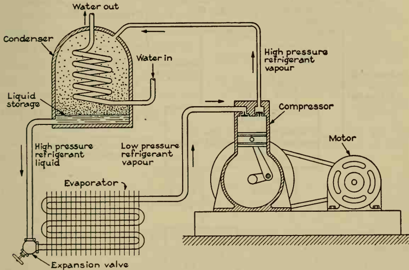
FIG. 92. Vapor compression air conditioning system. (Courtesy of the General Electric Air Conditioning Company.)
