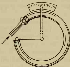
FIG. 66. The principle of the Bourdon gauge.
