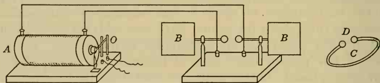
FIG. 258. Apparatus used by Hertz to demonstrate that electric oscillations produce electromagnetic waves.
