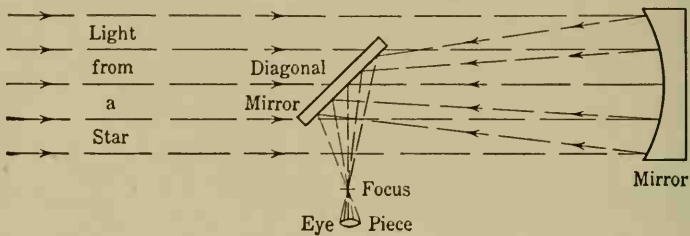
FIG. 6. The principle of the reflector. The diagonal mirror is relatively much smaller than shown in the diagram.
