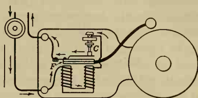
FIG. 244. An electric bell.
