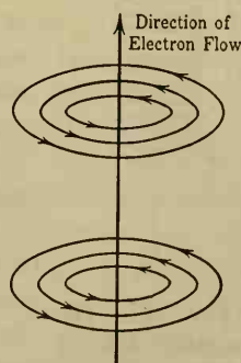
FIG. 241. The direction of lines of force of the magnetic field encircling a wire carrying an electric current.
