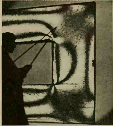
FIG. 197. A "map" of the stress distribution appears in transparent plastic models under load. (Courtesy of The Polaroid Corporation.)
