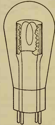
FIG. 261. A cylindrical plate, the invention of Sir John A. Fleming, arrested the electrons as they departed from the filament or cell sides and thus greatly increased the efficiency of the "electron valve."
