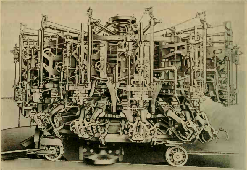
FIG. 107. Idealistic view of a 15-arm Owens bottle blowing machine. (Courtesy of the Owens-Illinois Glass Company.)
