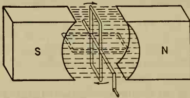
FIG. 251. Principle of a generator. A wire loop or coil cuts the lines of force between the poles N and S of a magnet.
