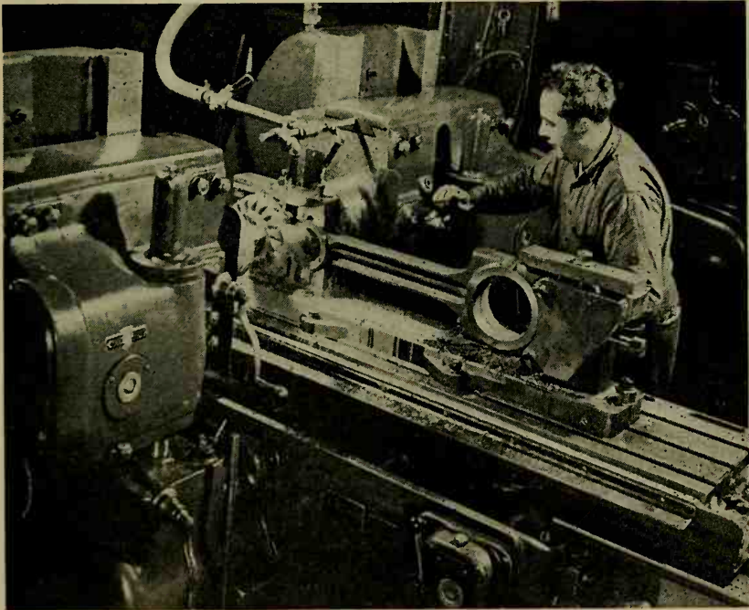
FIG. 106. A milling machine simultaneously finishing both sides of a large Diesel engine connecting rod. The two cutters have multiple teeth, similar to a circular saw. One of them is seen at the small end of the rod; the other is just behind it.
