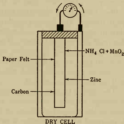
Fig. 282. Diagram of a dry cell.
