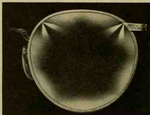
FIG. 196. Strains revealed by polarized light. (Courtesy of the American Optical Company.)
