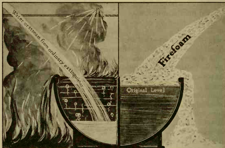
FIG. 284. Note how the foam floats on the liquid shutting off the oxygen and extinguishing the fire, and how the water goes to the bottom of the receptacle allowing the burning liquid to overflow and the fire to spread. (Courtesy of the American-La France and Foamite Industries, Inc.)
