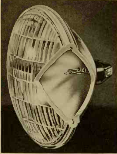
FIG. 205. An all-glass driving lamp, similar in construction to a sealed-beam headlight except that it employs one filament instead of two filaments. (Courtesy of the General Electric Company.)
