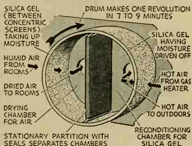
FIG. 94. How the Silica gel dehumidifier works. (Courtesy of Popular Science .)
