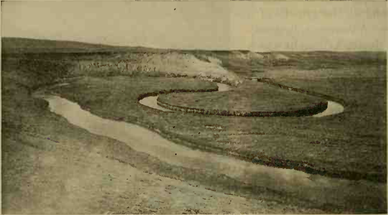
FIG. 41. The meanders of an old river. (Courtesy of the U. S. Geol. Survey.)
