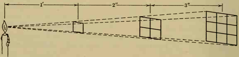
FIG. 215. Light intensity is inversely proportional to the square of the distance from the source.
