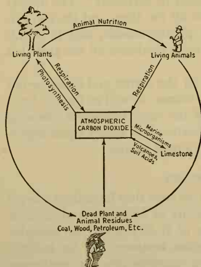
FIG. 308. The carbon dioxide cycle in nature.
