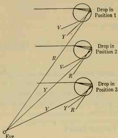
FIG. 182. How a rainbow is produced.
