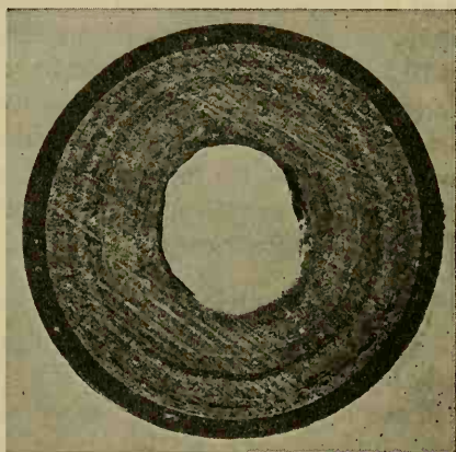
FIG. 320. Scale produced in a pipe by hard water. (Courtesy of the Permutit Company.)
