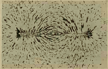
FIG. 225. Lines of force of a rod magnet as shown by iron filings placed on a sheet of paper above the magnet.
