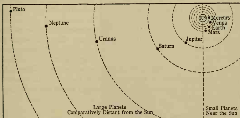
FIG. 23. The relative distances of the planets from the sun.
