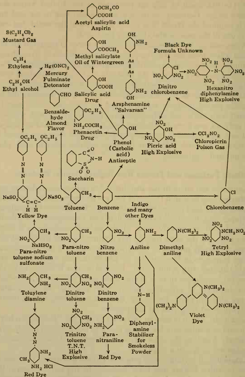
FIG. 302. A few of the interrelationships among aromatic chemical compounds.
