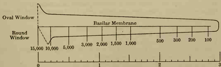
FIG. 220. The inner ear straightened out. (After Fletcher.)
