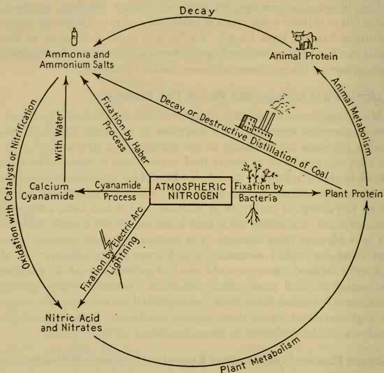
FIG. 286. The nitrogen cycle in nature.
