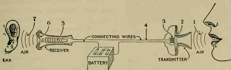
FIG. 248. The simplest telephone circuit. (Courtesy of the American Telephone and Telegraph Company.)
