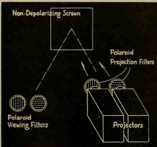
FIG. 198. The principle of the three-dimensional motion pictures using Polaroid filters. (Courtesy of The Polaroid Corporation.)
