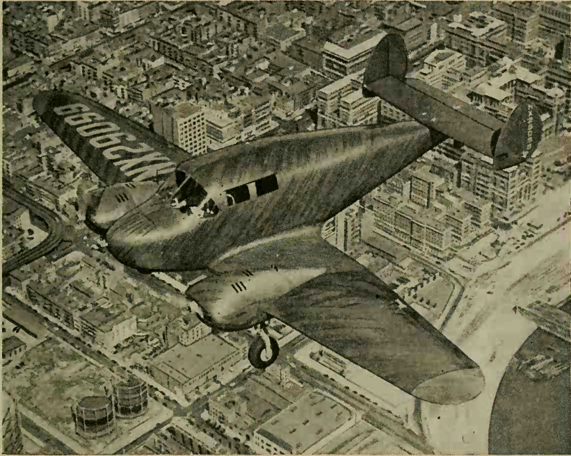
FIG. 154. Plastic-plywood plane. (Courtesy of the Langley Aviation Corporation.)
