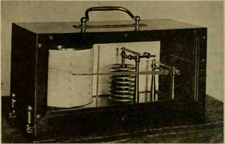
FIG. 86. The aneroid barograph. (Courtesy of the U. S. Weather Bureau.)
