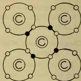
FIG. 278. Carbon atoms share pairs of electrons.
