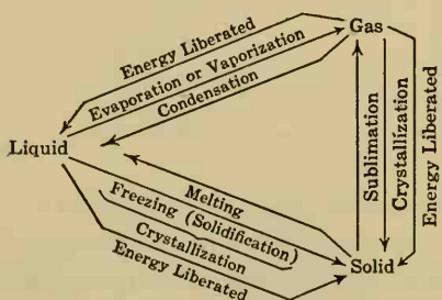
FIG. 70. The chief physical processes.
