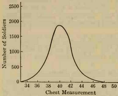
FIG. 73A. The curve of variation of the chest measurements of Scottish soldiers.
