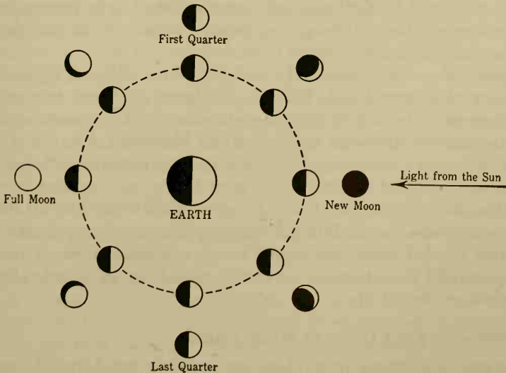
FIG. 27. The phases of the moon.
