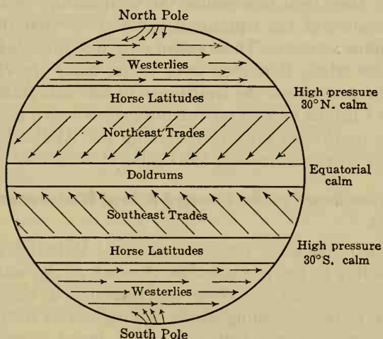
FIG. 75. The most important prevailing winds on the earth.
