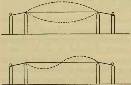
FIG. 216. The pitch is determined by the number of vibrations per second.
