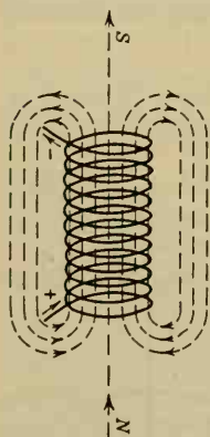
FIG. 243. The magnetic field of a helix.
