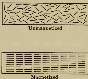
FIG. 227. The molecules are thought to be oriented when the bar of iron is magnetized. The molecules in the unmagnetized bar are not oriented, while those in the magnetized bar are oriented.
